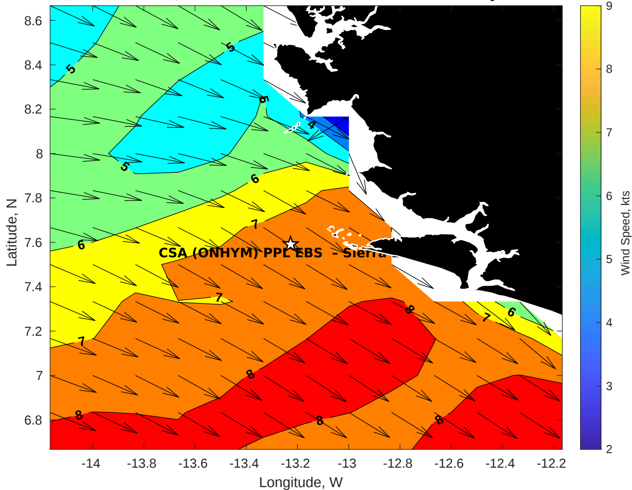
GFS Winds (kts) for CSA (ONHYM) PPL EBS - Sierra Leone at 30-Jan-2026 09:00:00
