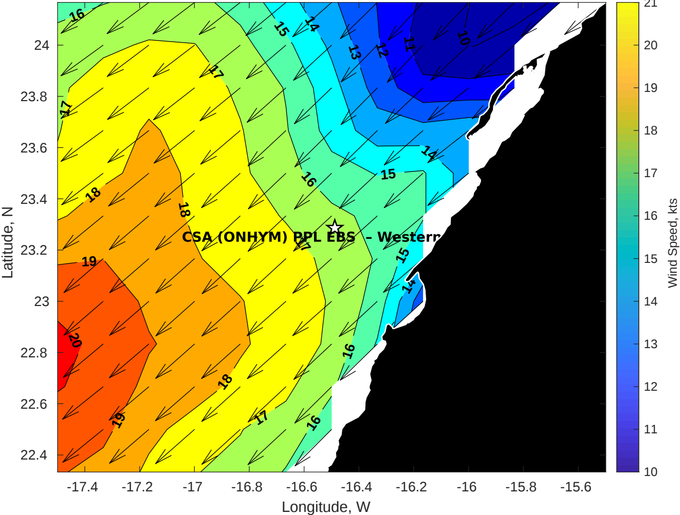
GFS Winds (kts) for CSA (ONHYM) PPL EBS - Western Sahara at 30-Jan-2026 09:00:00
