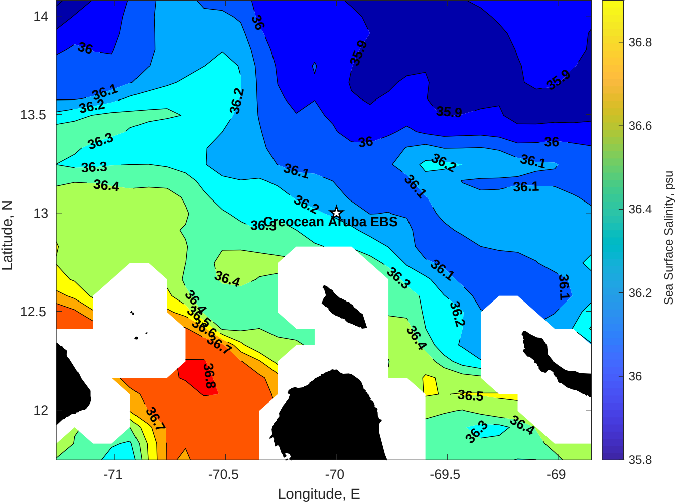
Surface Salinity for Creocan Aruba EBS at 29-Jan-2026 00:00:00
