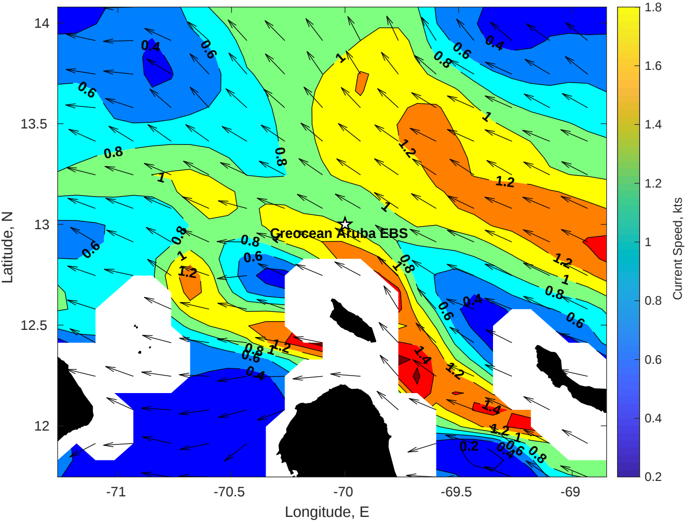
Surface Currents for Creocean Aruba EBS at 29-Jan-2026 00:00:00
