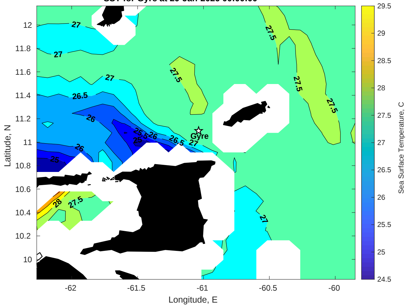
SST for Gyre at 29-Jan-2026 00:00:00
