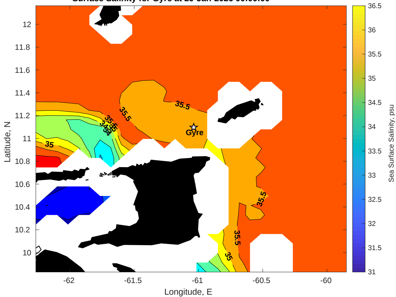
Surface Salinity for Gyre at 29-Jan-2026 00:00:00
