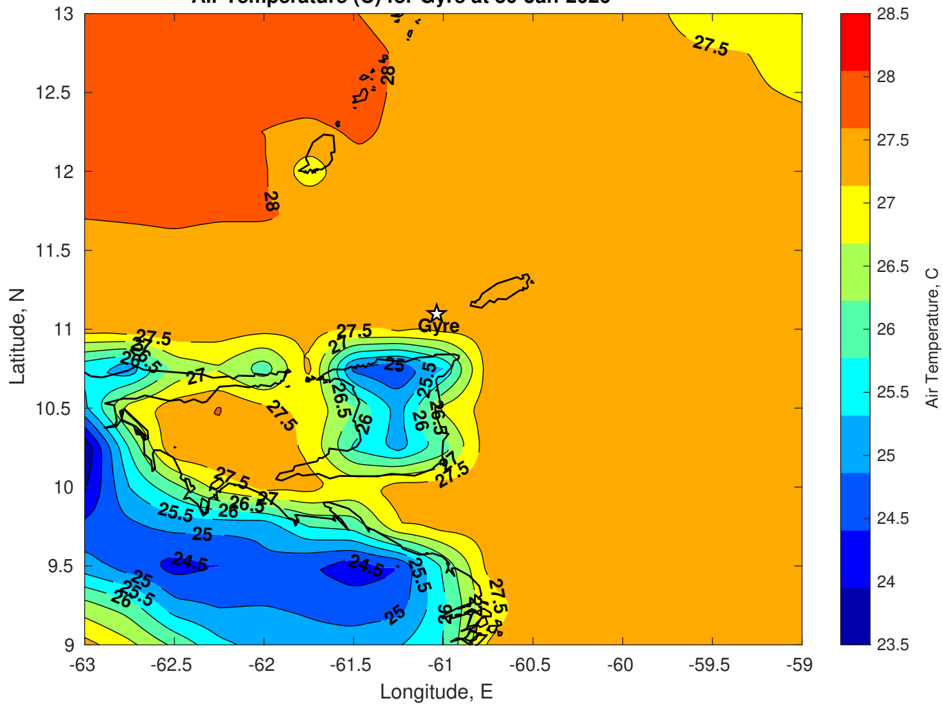
Air Temperature (C) for Gyre at 30-Jan-2026
