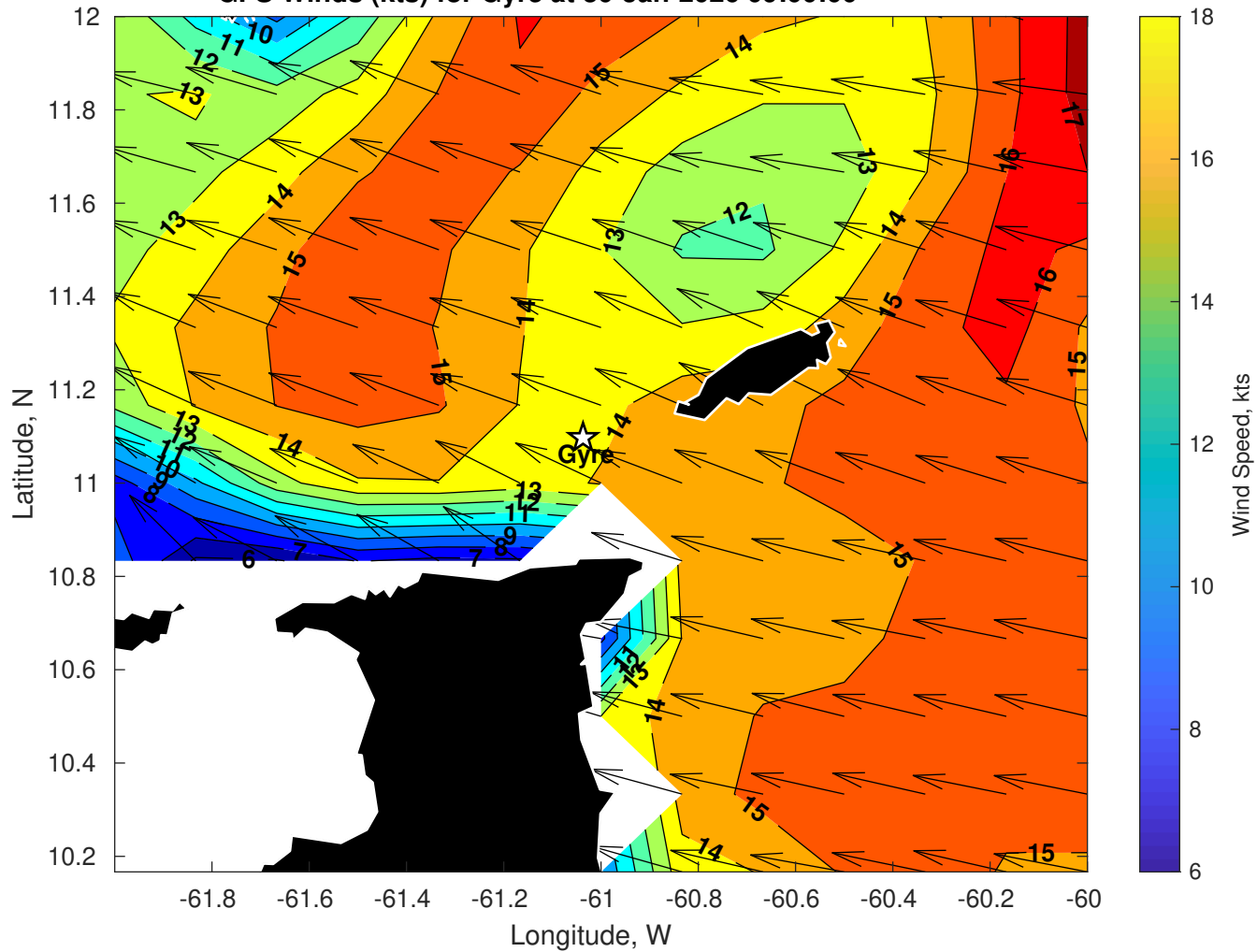
GFS Winds (kts) for Gyre at 30-Jan-2026 09:00:00
