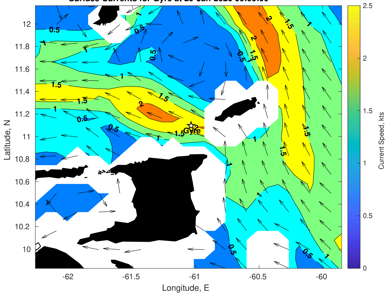
Surface Currents for Gyre at 29-Jan-2026 00:00:00
