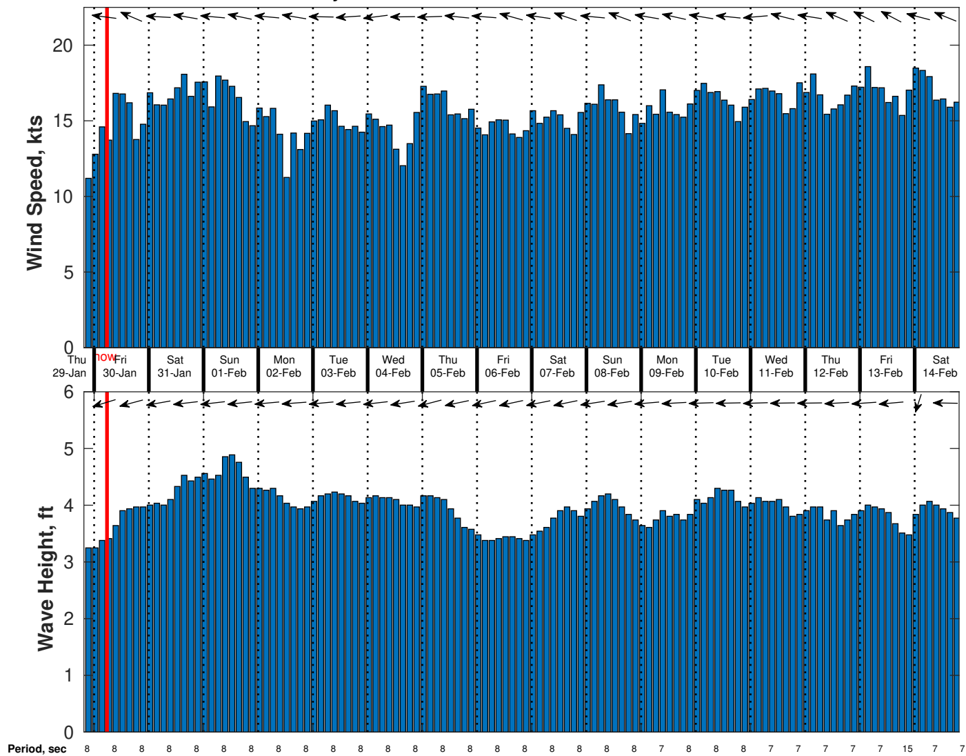
Wind & Wave Forecast for Gyre from 29-Jan-2026 20:00:00 to 14-Feb-2026 20:00:00
