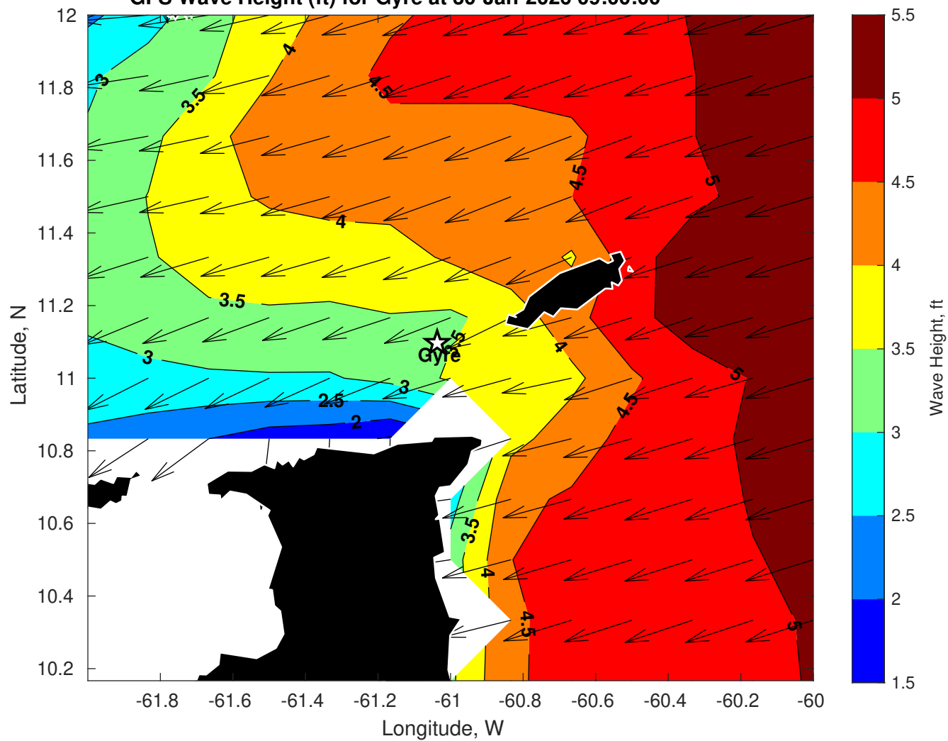
GFS Wave Height (ft) for Gyre at 30-Jan-2026 09:00:00
