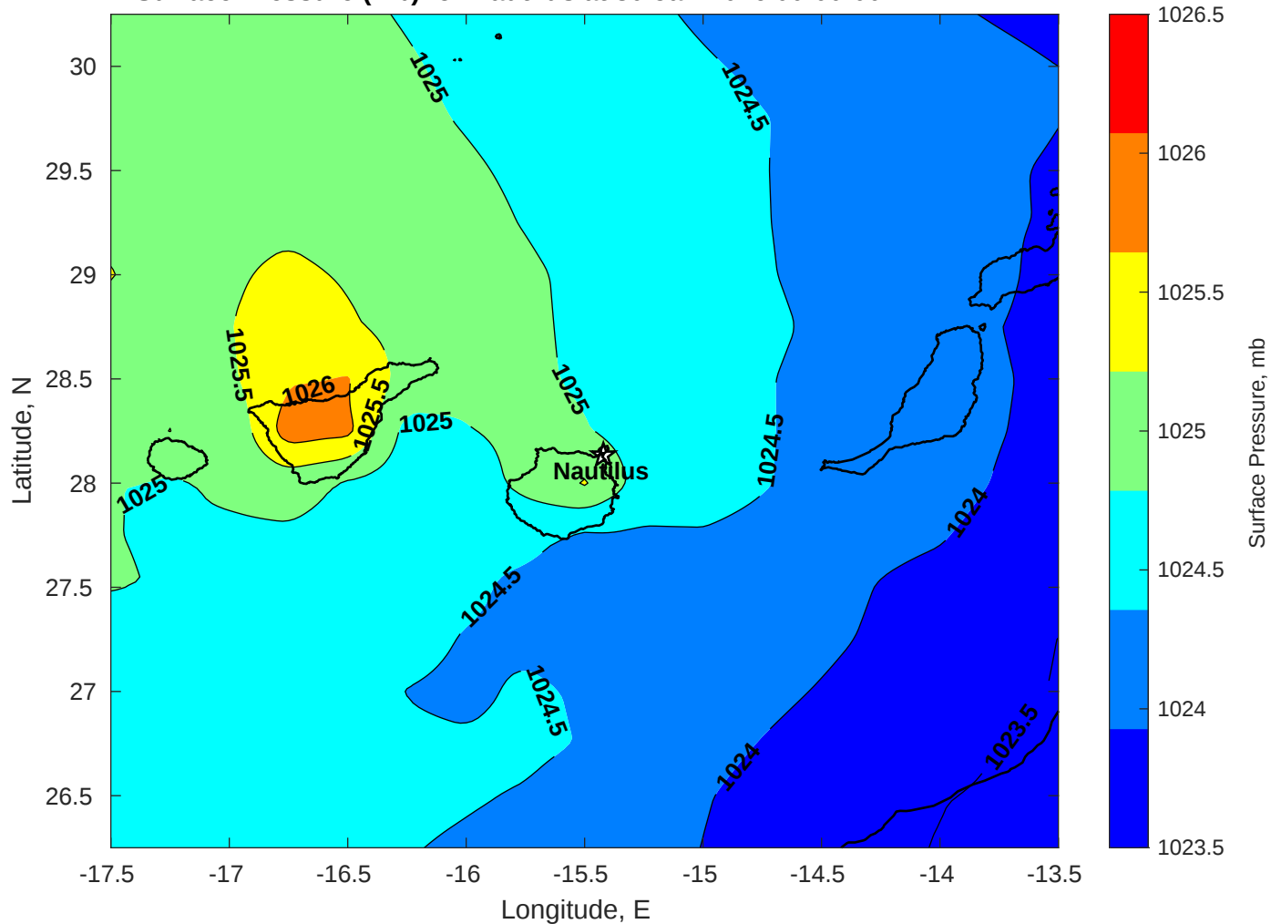
Surface Pressure (mb) for Nautilus at 30-Jan-2026 00:00:00
