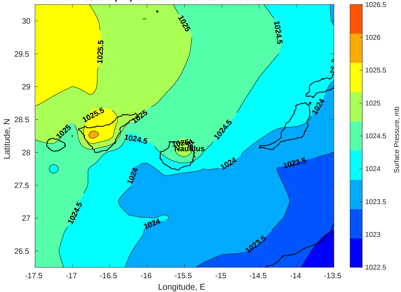
Surface Pressure (mb) for Nautilus at 31-Jan-2026 00:00:00
