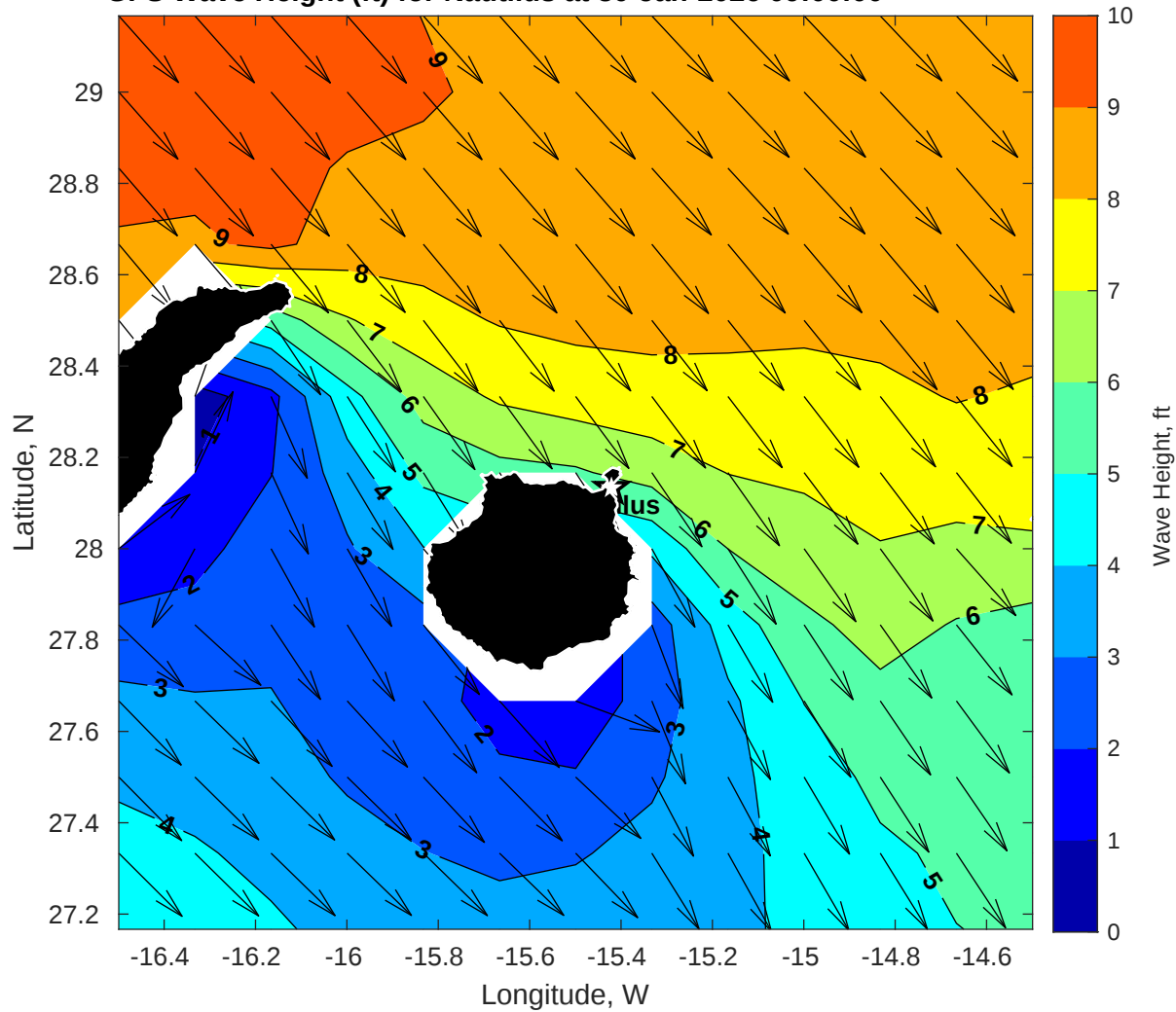
GFS Wave Height (ft) for Nautilus at 30-Jan-2026 09:00:00
