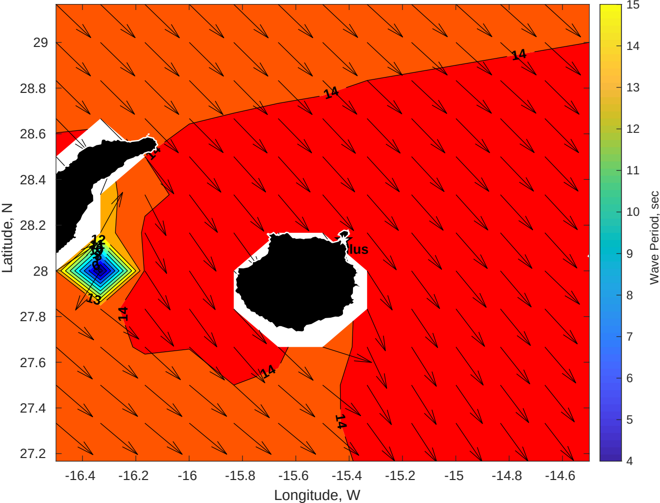
GFS Wave Period (sec) for Nautilus at 30-Jan-2026 09:00:00
