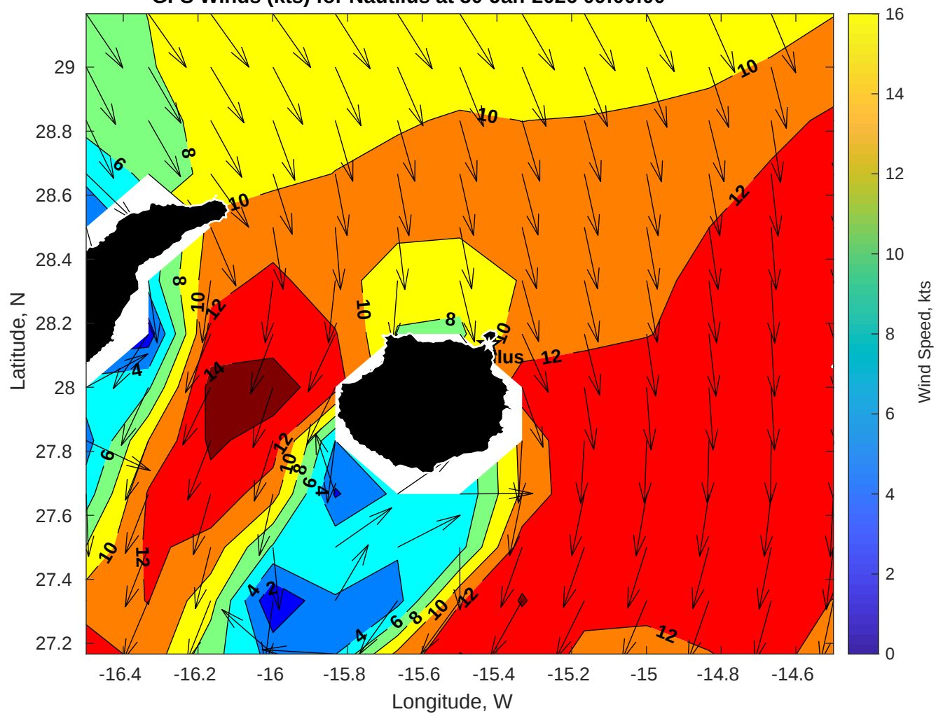
GFS Winds (kts) for Nautilus at 30-Jan-2026 09:00:00
