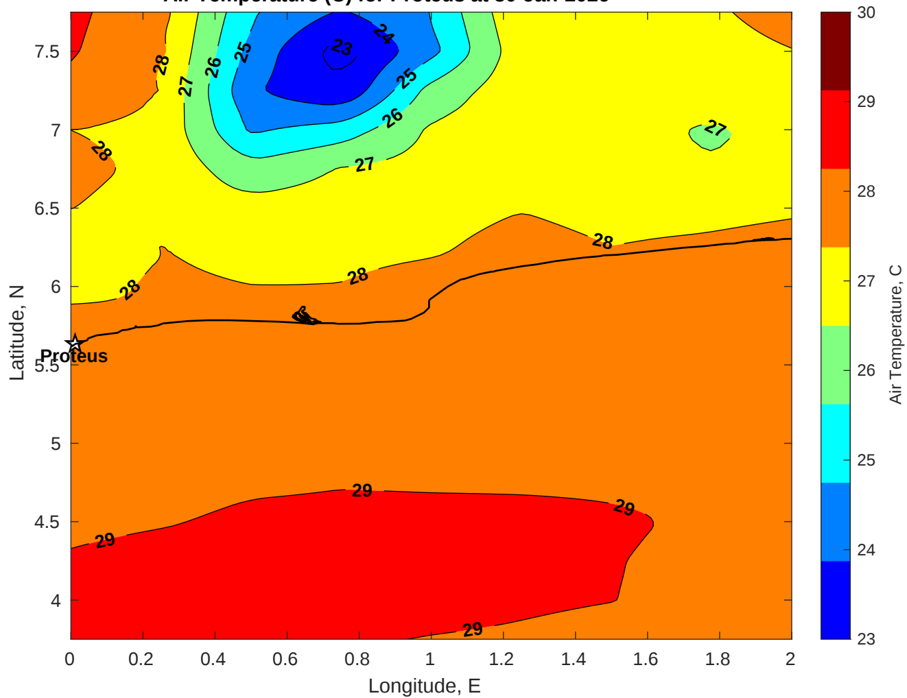
Air Temperature (C) for Proteus at 30-Jan-2026
