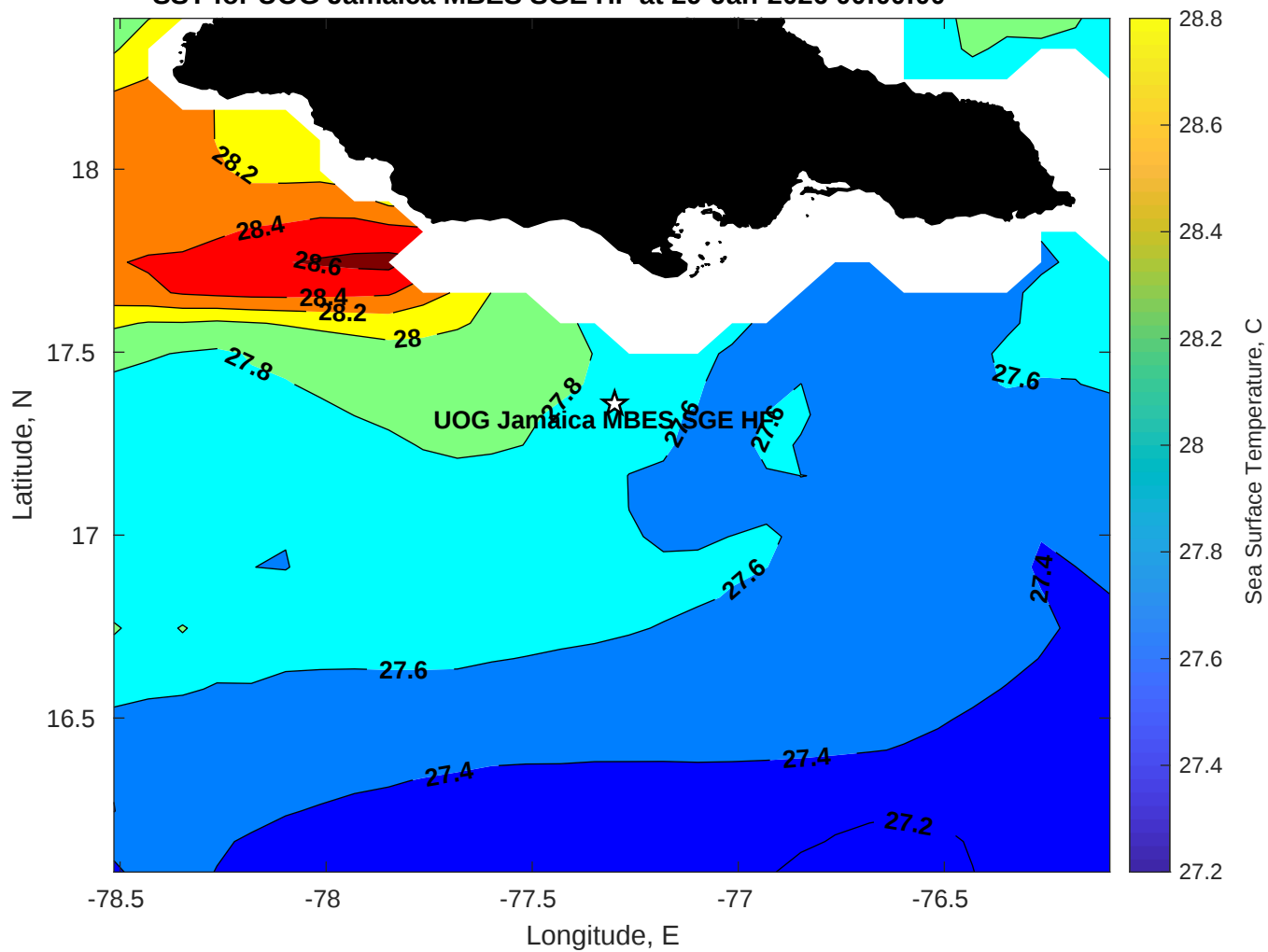
SST for UOG Jamaica MBES SGE HF at 29-Jan-2026 00:00:00
