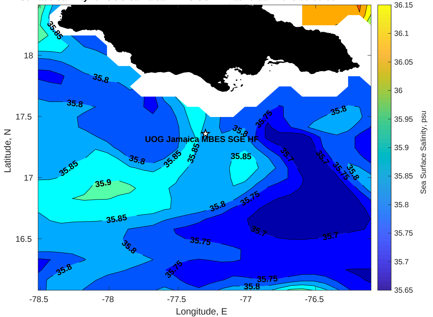
Surface Salinity for UOG Jamaica MBES SGE HF at 29-Jan-2026 00:00:00
