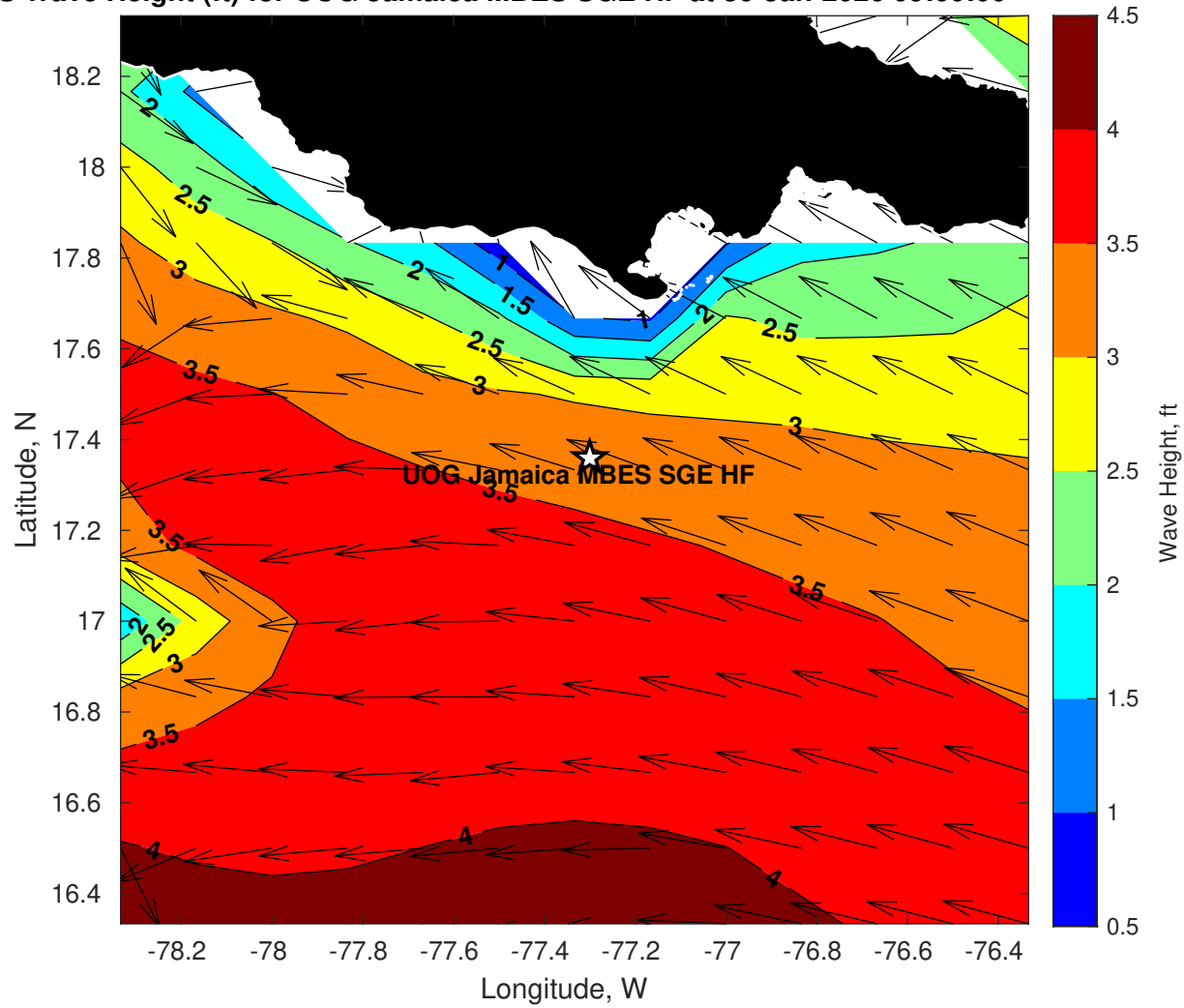
GFS Wave Height (ft) for UOG Jamaica MBES SGE HF at 30-Jan-2026 09:00:00
