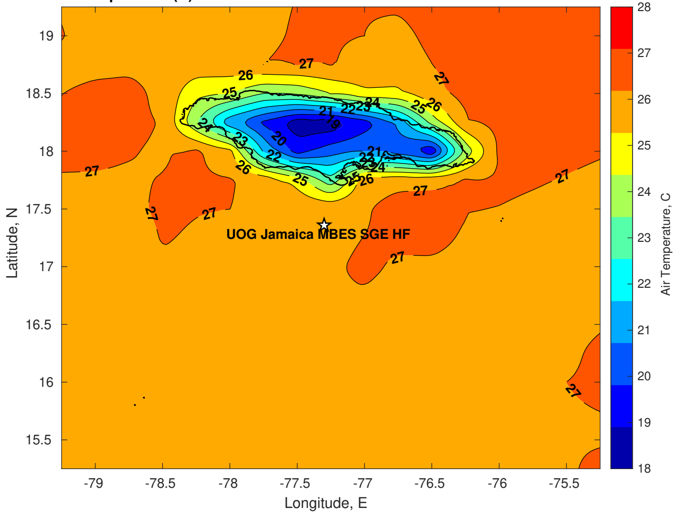
Air Temperature (C) for UOG Jamaica MBES SGE HF at 30-Jan-2026
