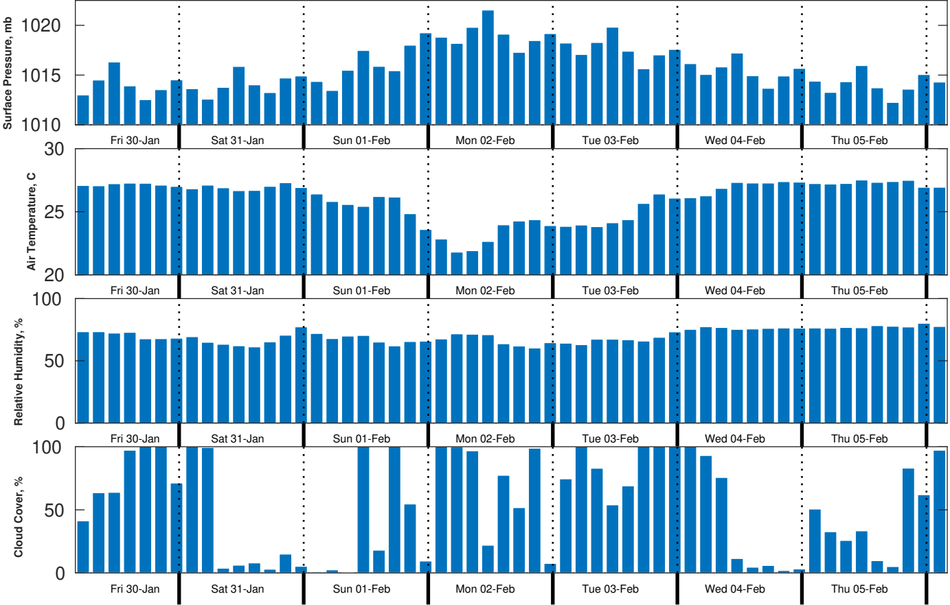
Met Forecast for UOG Jamaica MBES SGE HF from 30-Jan-2026 06:00:00 to 06-Feb-2026 06:00:00
