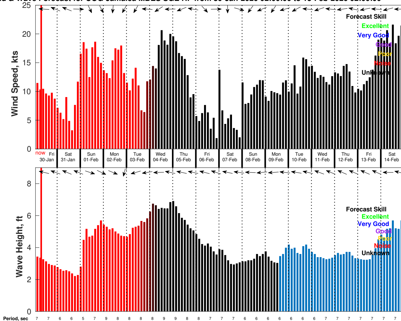
Wind & Wave Forecast for UOG Jamaica MBES SGE HF from 30-Jan-2026 02:00:00 to 15-Feb-2026 02:00:00
