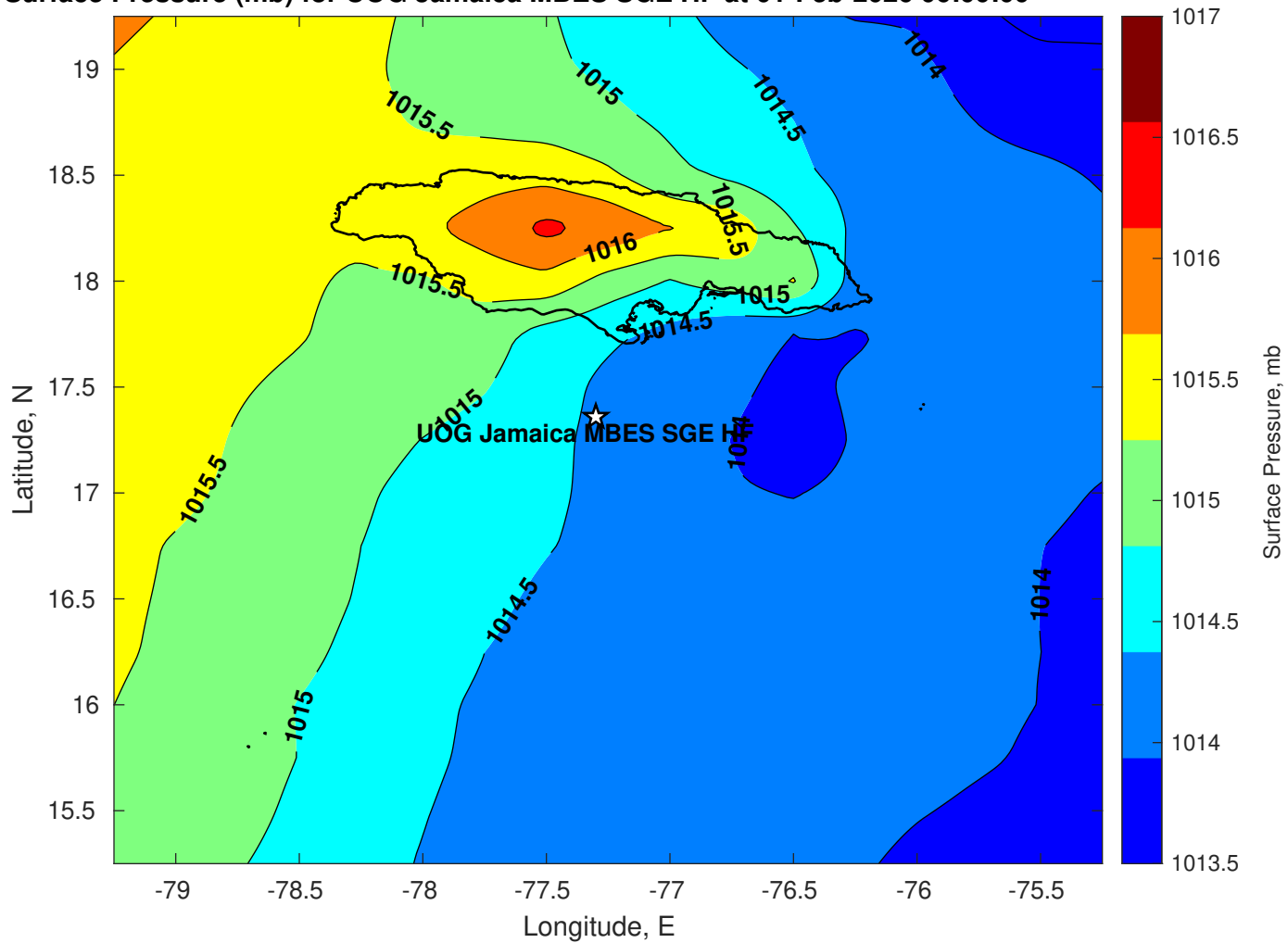
Surface Pressure (mb) for UOG Jamaica MBES SGE HF at 01-Feb-2026 06:00:00
