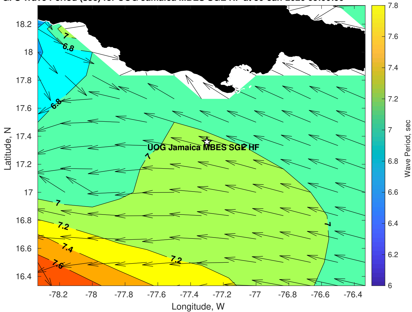
GFS Wave Period (sec) for UOG Jamaica MBES SGE HF at 30-Jan-2026 09:00:00
