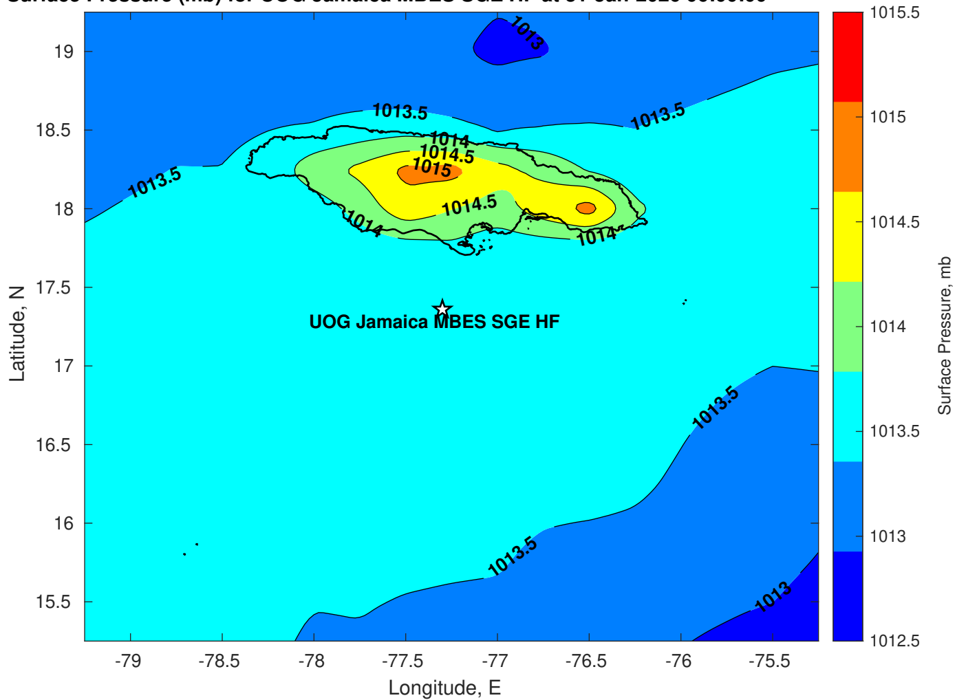
Surface Pressure (mb) for UOG Jamaica MBES SGE HF at 31-Jan-2026 06:00:00
