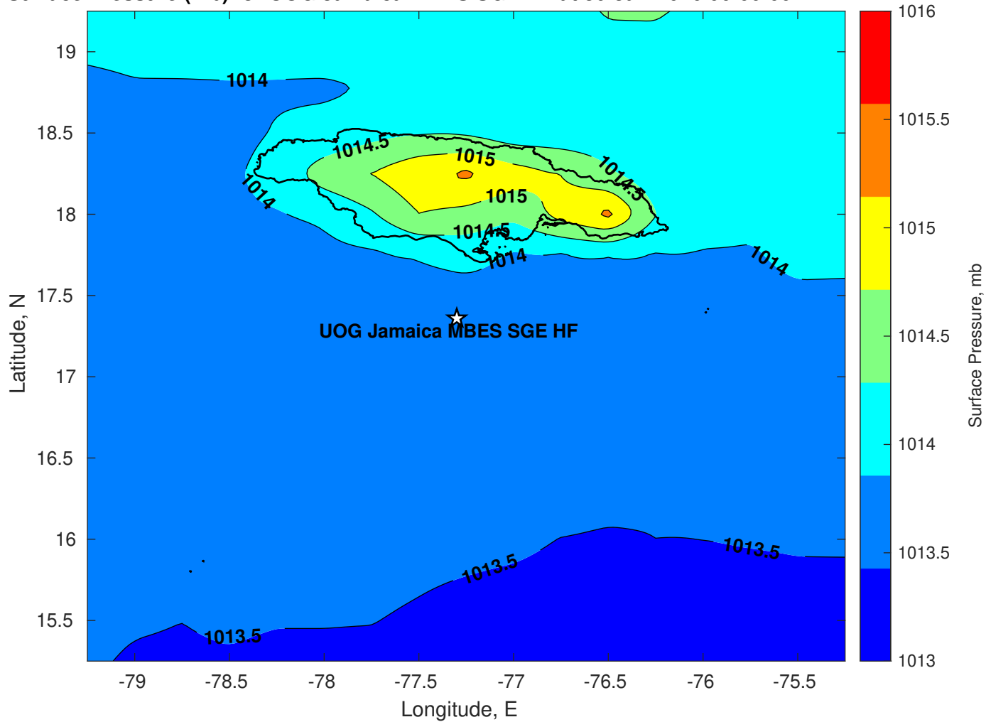
Surface Pressure (mb) for UOG Jamaica MBES SGE HF at 30-Jan-2026 06:00:00
