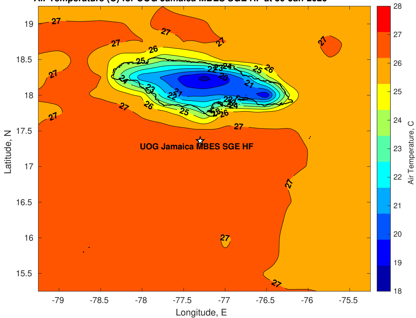
Air Temperature (C) for UOG Jamaica MBES SGE HF at 30-Jan-2026
