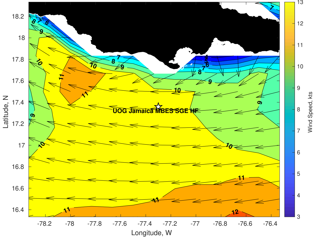
GFS Winds (kts) for UOG Jamaica MBES SGE HF at 30-Jan-2026 09:00:00
