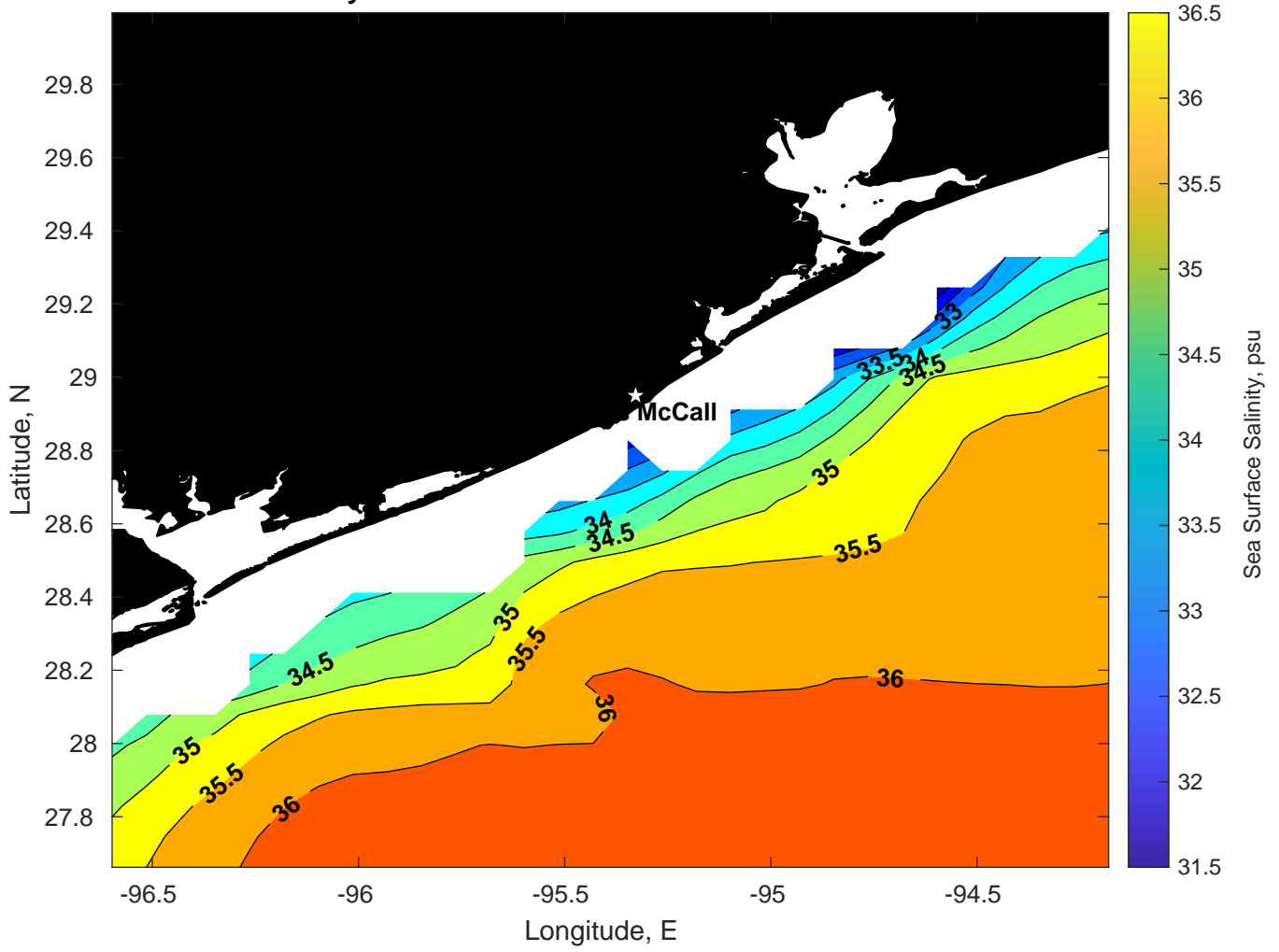
Surface Salinity for Brooks McCall at 30-Jan-2026 00:00:00
