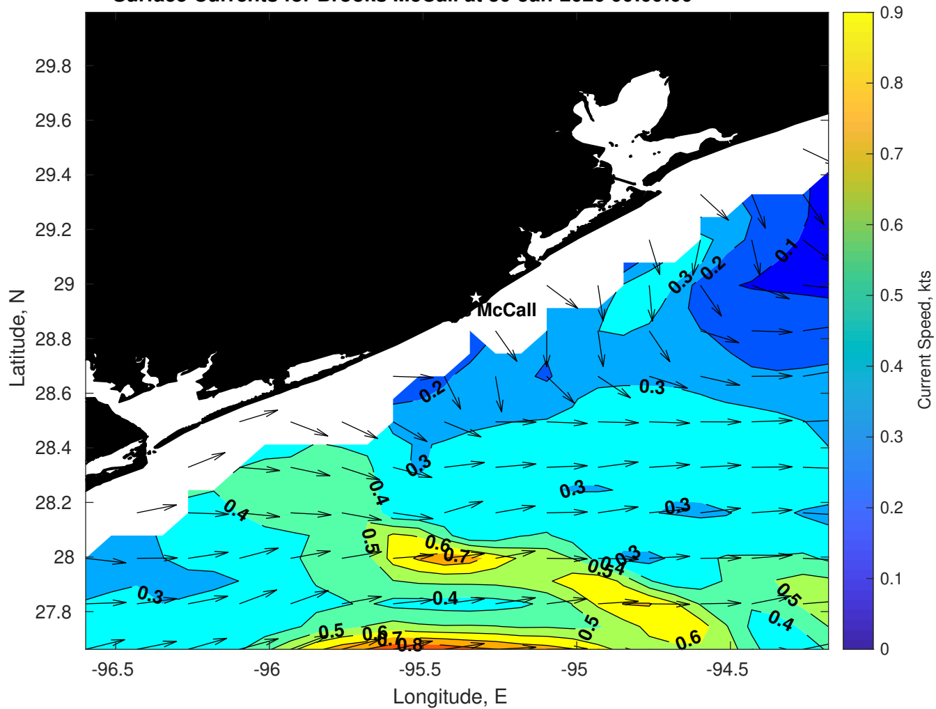
Surface Currents for Brooks McCall at 30-Jan-2026 00:00:00
