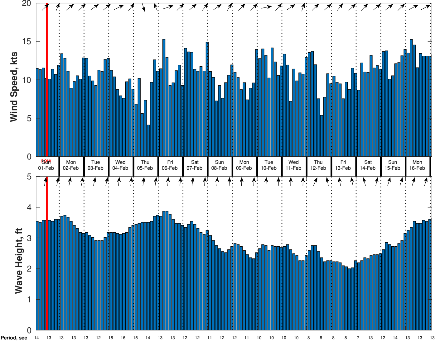
Wind & Wave Forecast for CSA (ONHYM) PPL EBS - Cote d'Ivoire from 31-Jan-2026 01:00:00 to 16-Feb-2026 01:00:00
