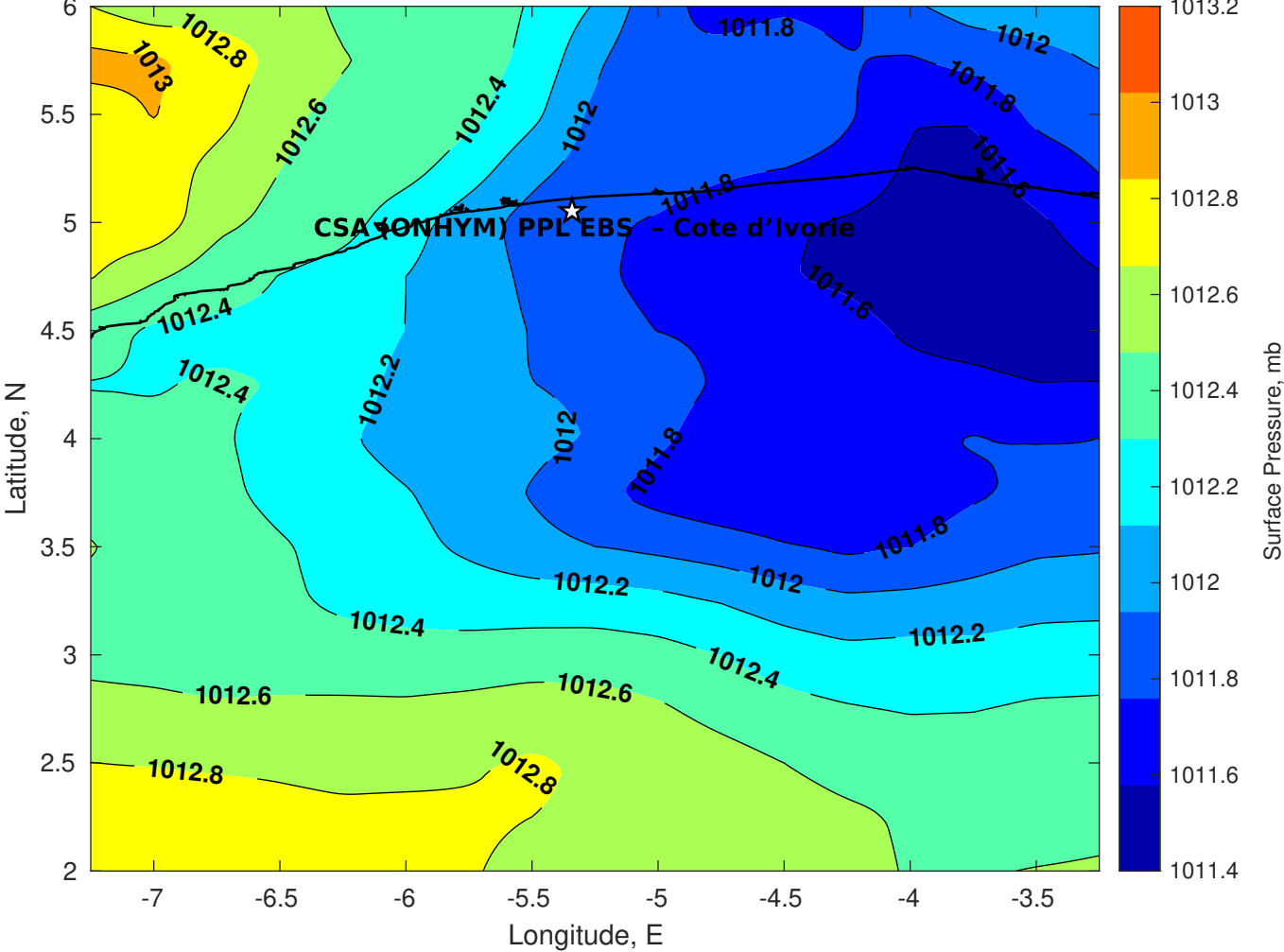
Surface Pressure (mb) for CSA (ONHYM) PPL EBS - Cote d'Ivoire at 01-Feb-2026 00:00:00
