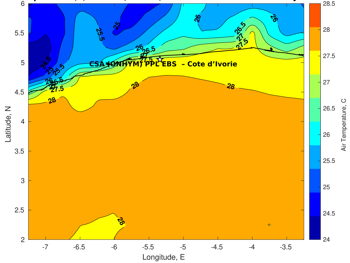
Air Temperature (C) for CSA (ONHYM) PPL EBS - Cote d'Ivoire at 31-Jan-2026
