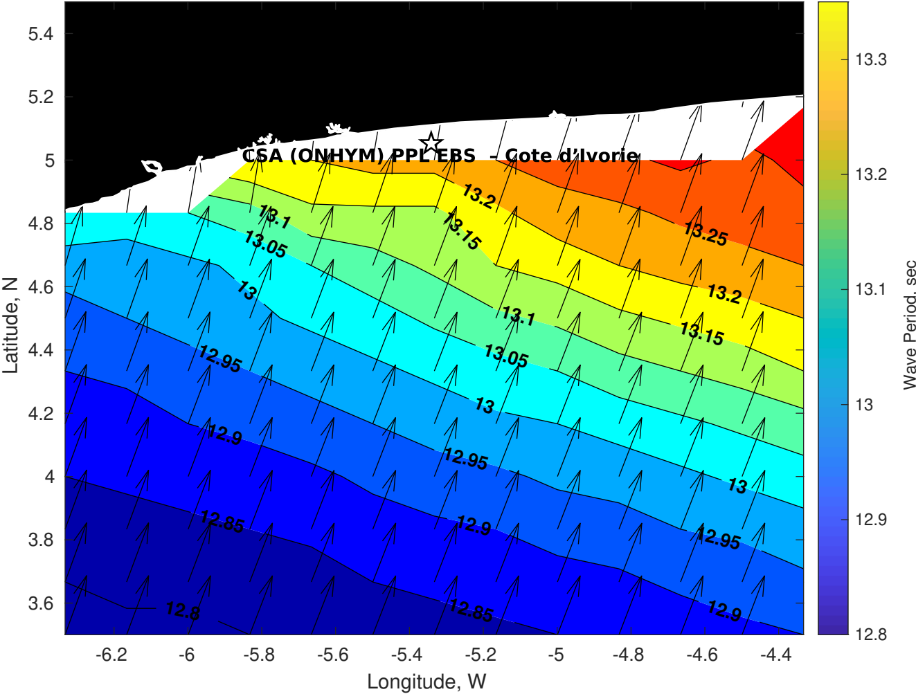
GFS Wave Period (sec) for CSA (ONHYM) PPL EBS - Cote d'Ivoire at 31-Jan-2026 09:00:00
