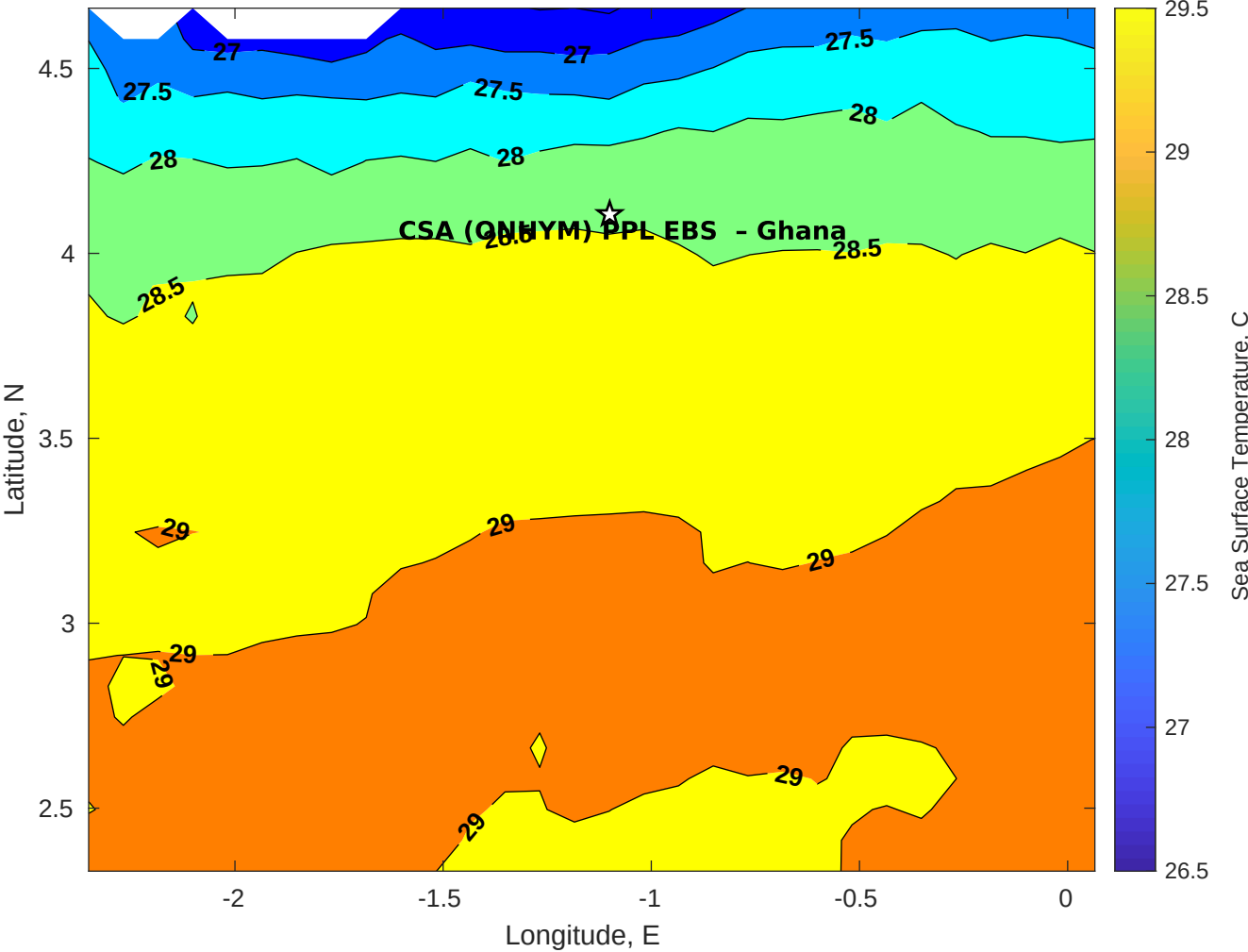
SST for CSA (ONHYM) PPL EBS - Ghana at 30-Jan-2026 00:00:00
