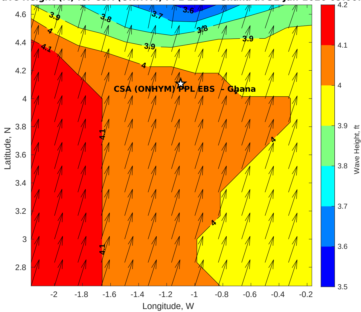
GFS Wave Height (ft) for CSA (ONHYM) PPL EBS - Ghana at 31-Jan-2026 09:00:00
