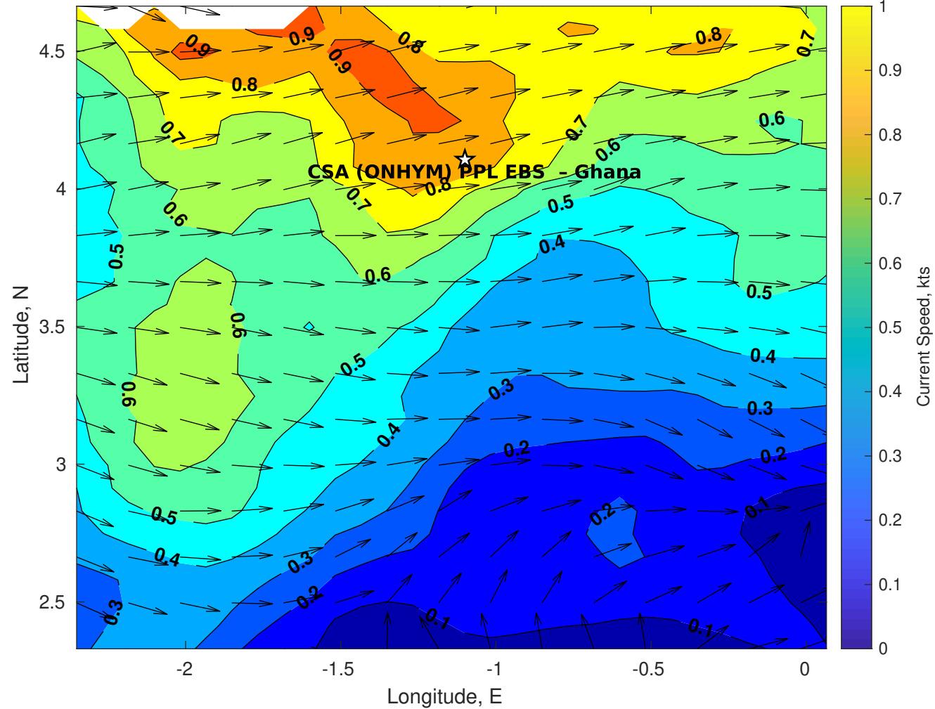
Surface Currents for CSA (ONHYM) PPL EBS - Ghana at 30-Jan-2026 00:00:00
