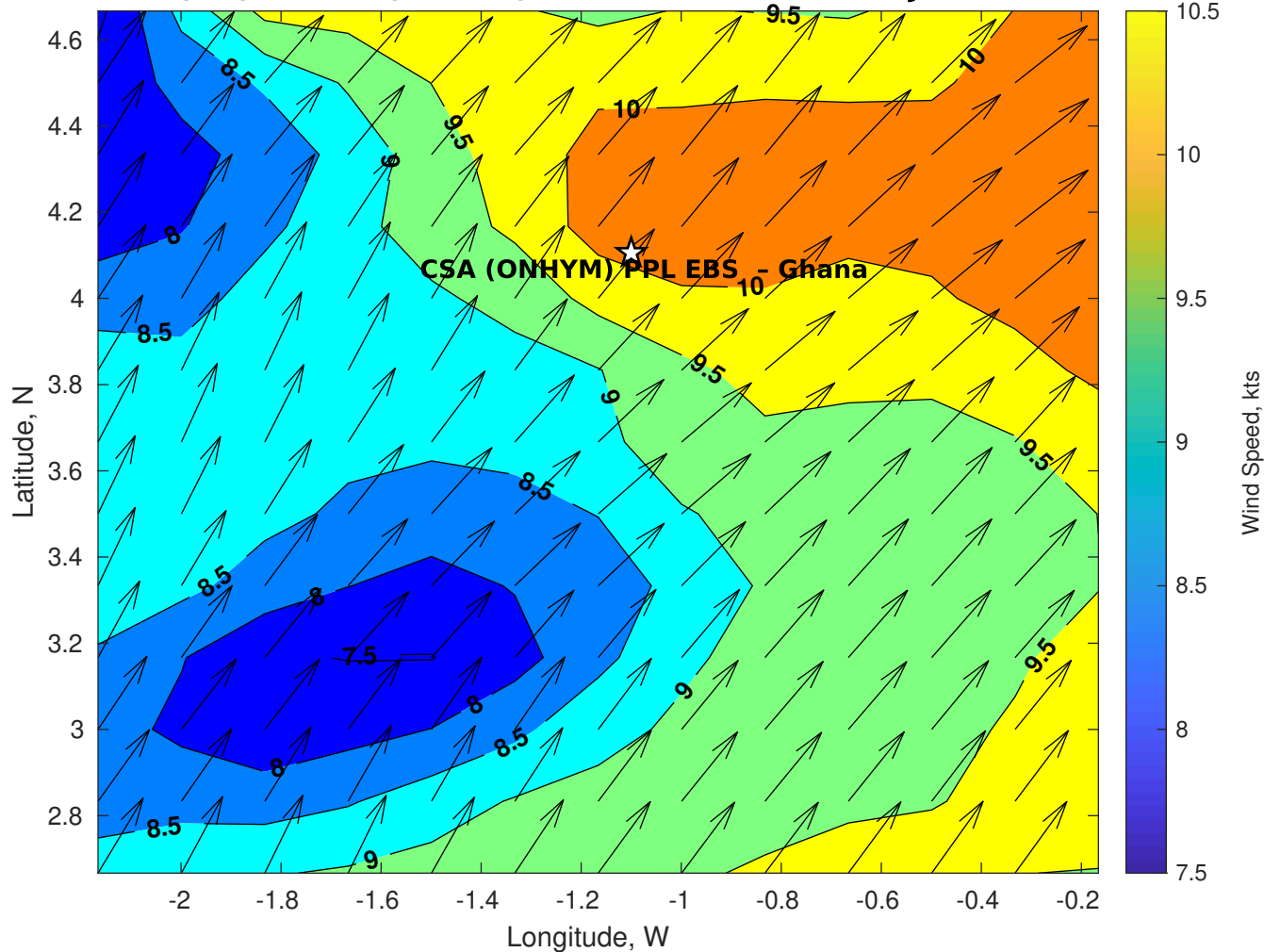
GFS Winds (kts) for CSA (ONHYM) PPL EBS - Ghana at 31-Jan-2026 09:00:00
