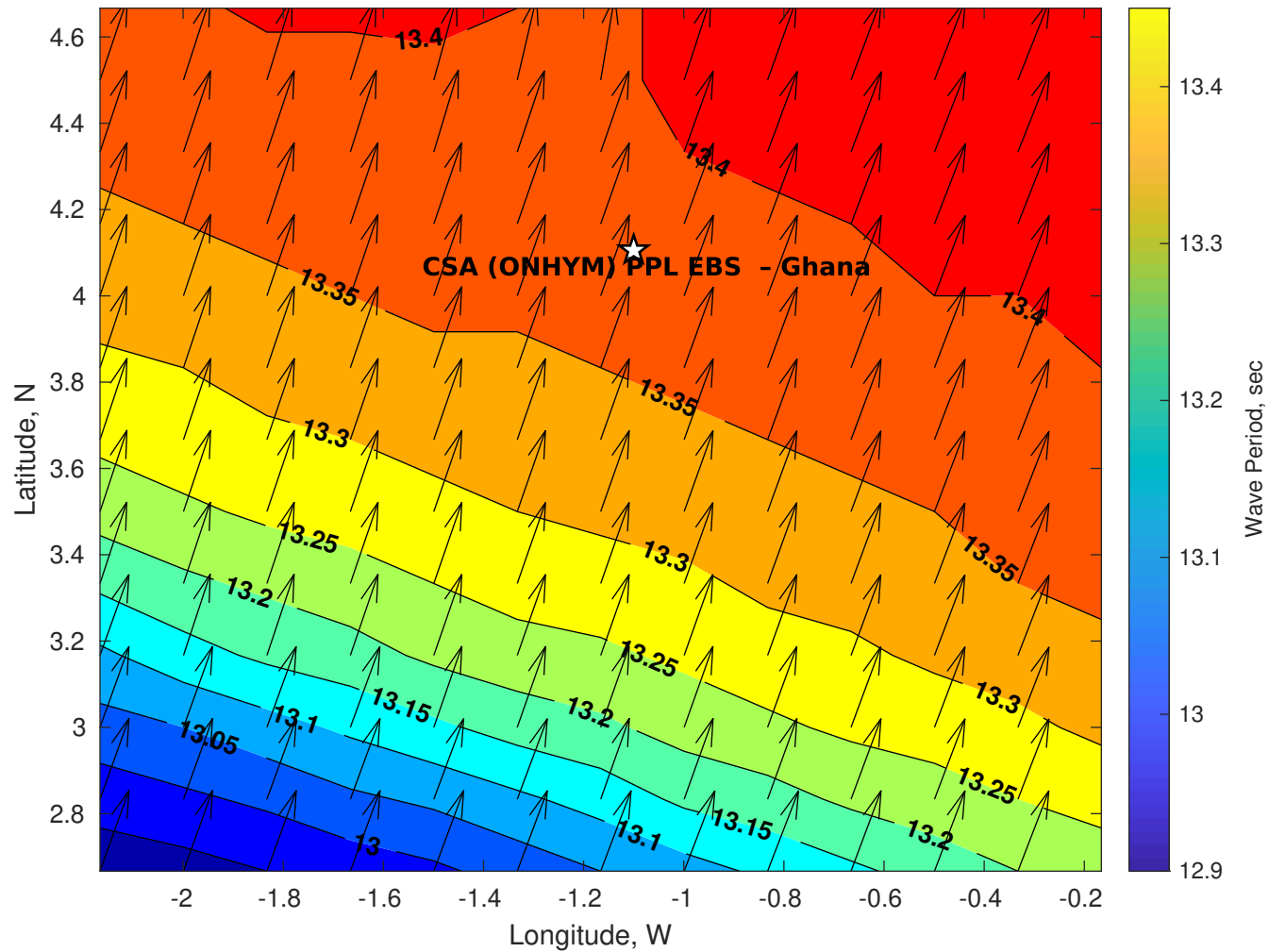
GFS Wave Period (sec) for CSA (ONHYM) PPL EBS - Ghana at 31-Jan-2026 09:00:00
