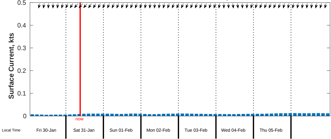
Surface Current Forecast for CSA (ONHYM) PPL EBS - Ghana from 30-Jan-2026 00:00:00 to 07-Feb-2026 00:00:00
