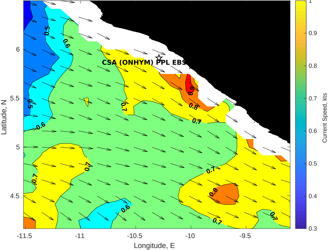
Surface Currents for CSA (ONHYM) PPL EBS - Liberia at 30-Jan-2026 00:00:00
