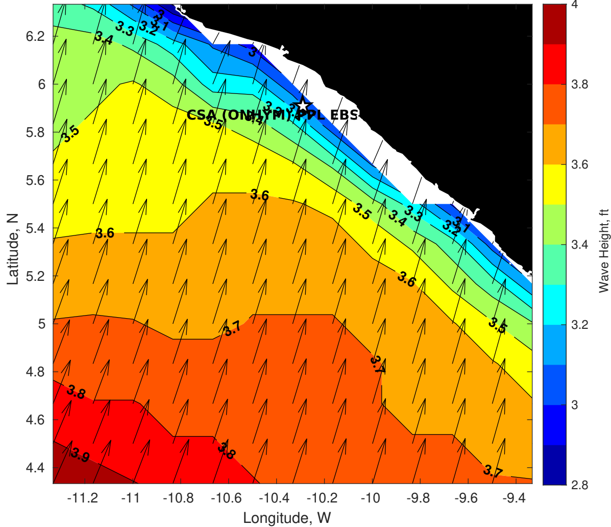
GFS Wave Height (ft) for CSA (ONHYM) PPL EBS - Liberia at 31-Jan-2026 09:00:00
