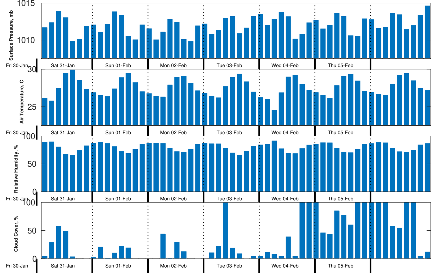
Met Forecast for CSA (ONHYM) PPL EBS - Liberia from 31-Jan-2026 00:00:00 to 07-Feb-2026 00:00:00
