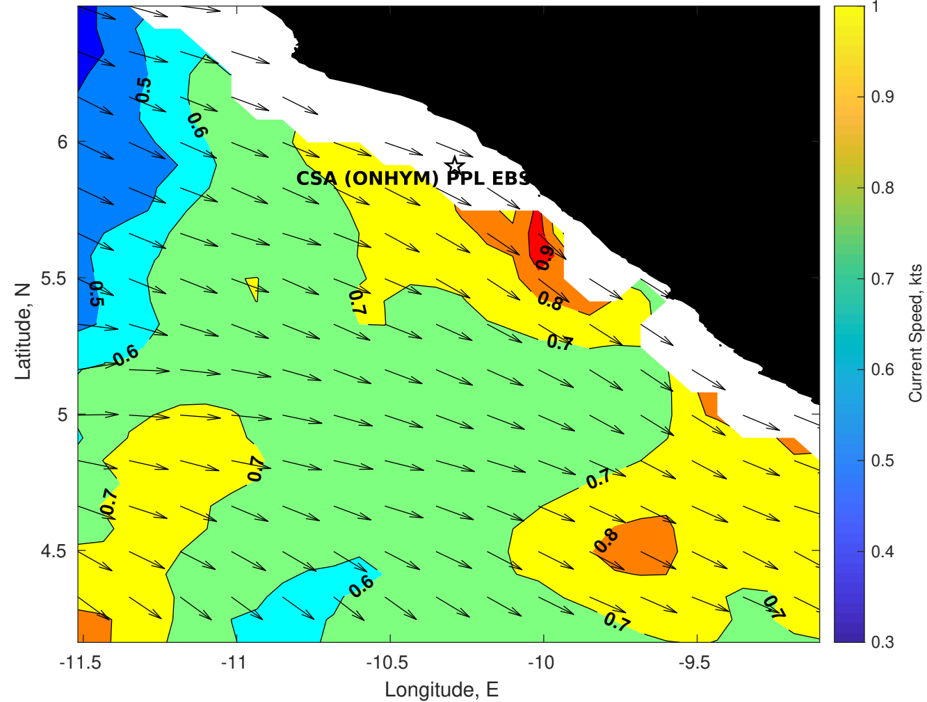
Surface Currents for CSA (ONHYM) PPL EBS - Liberia at 30-Jan-2026 00:00:00
