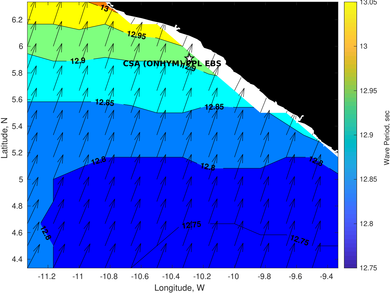
GFS Wave Period (sec) for CSA (ONHYM) PPL EBS - Liberia at 31-Jan-2026 09:00:00
