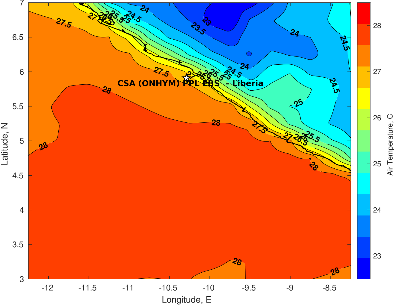
Air Temperature (C) for CSA (ONHYM) PPL EBS - Liberia at 31-Jan-2026
