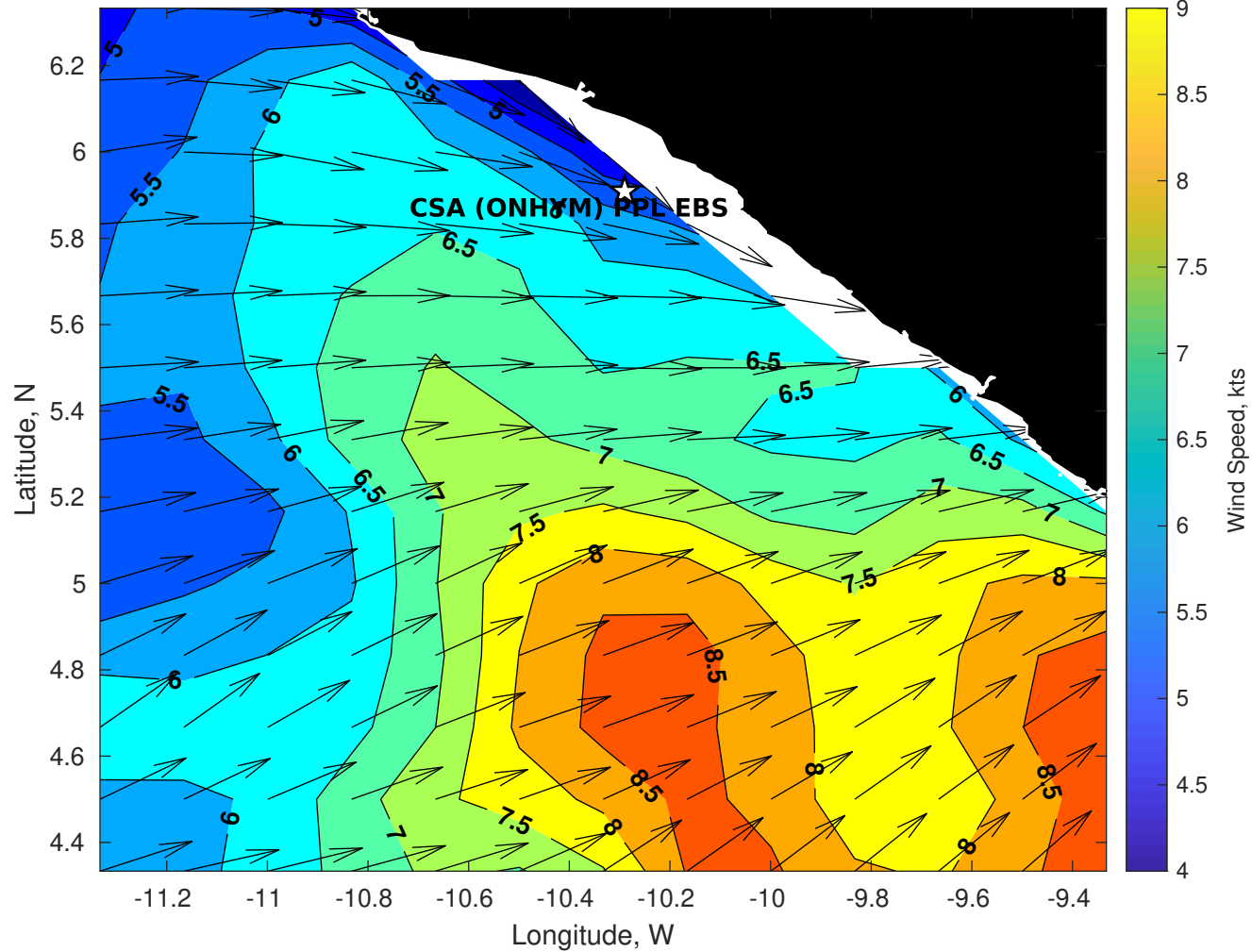
GFS Winds (kts) for CSA (ONHYM) PPL EBS - Liberia at 31-Jan-2026 09:00:00
