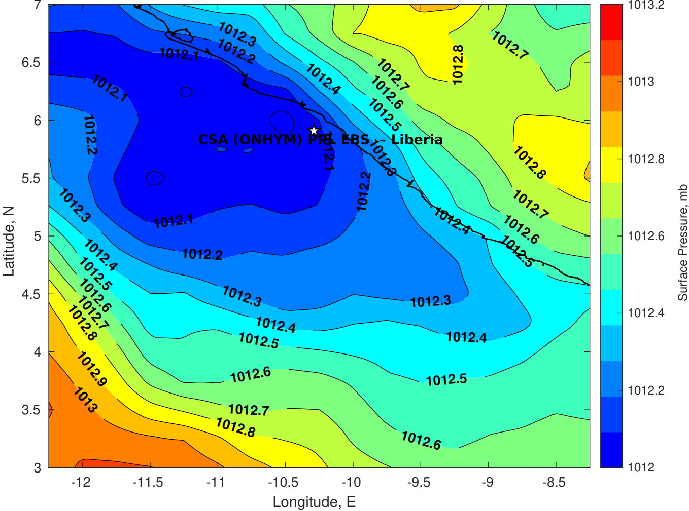
Surface Pressure (mb) for CSA (ONHYM) PPL EBS - Liberia at 01-Feb-2026 00:00:00
