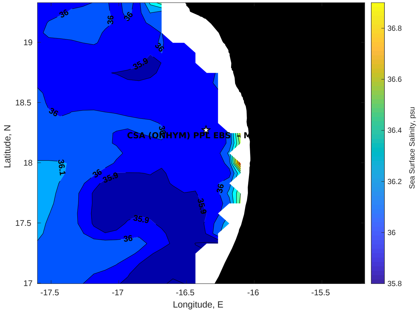
Surface Salinity for CSA (ONHYM) PPL EBS - Mauritania at 30-Jan-2026 00:00:00
