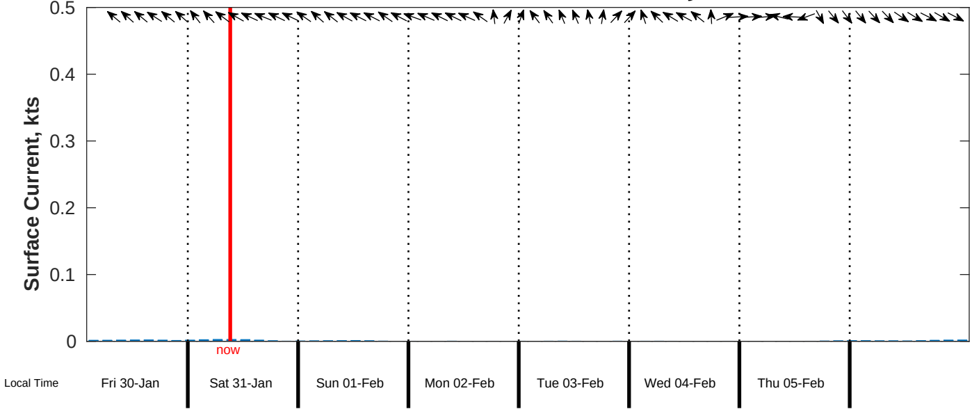
Surface Current Forecast for CSA (ONHYM) PPL EBS - Mauritania from 30-Jan-2026 00:00:00 to 07-Feb-2026 00:00:00
