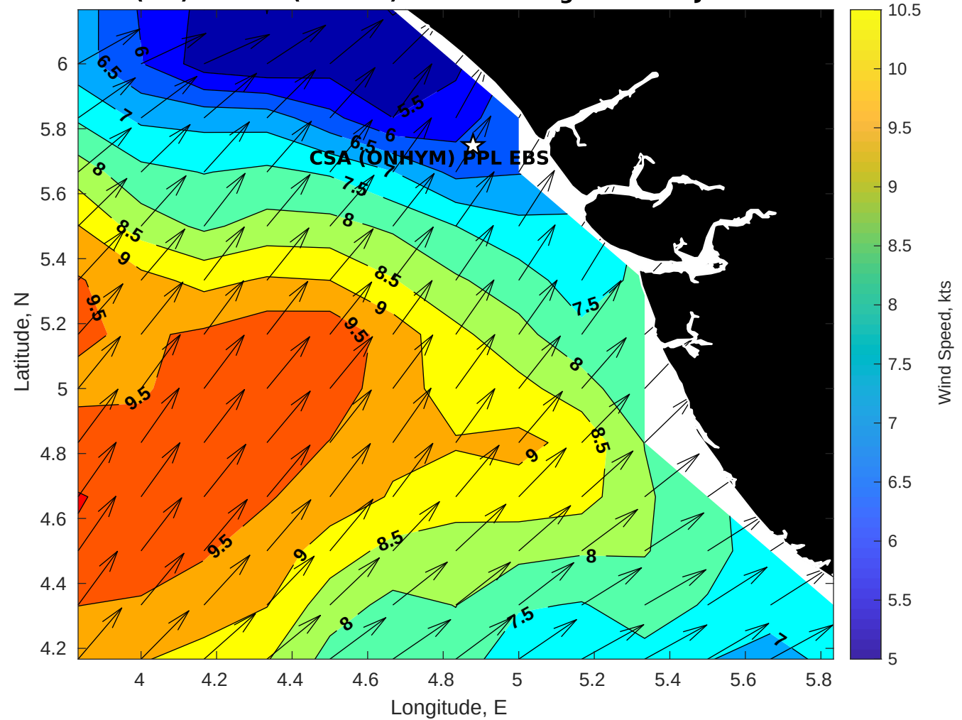
GFS Winds (kts) for CSA (ONHYM) PPL EBS - Nigeria at 31-Jan-2026 09:00:00
