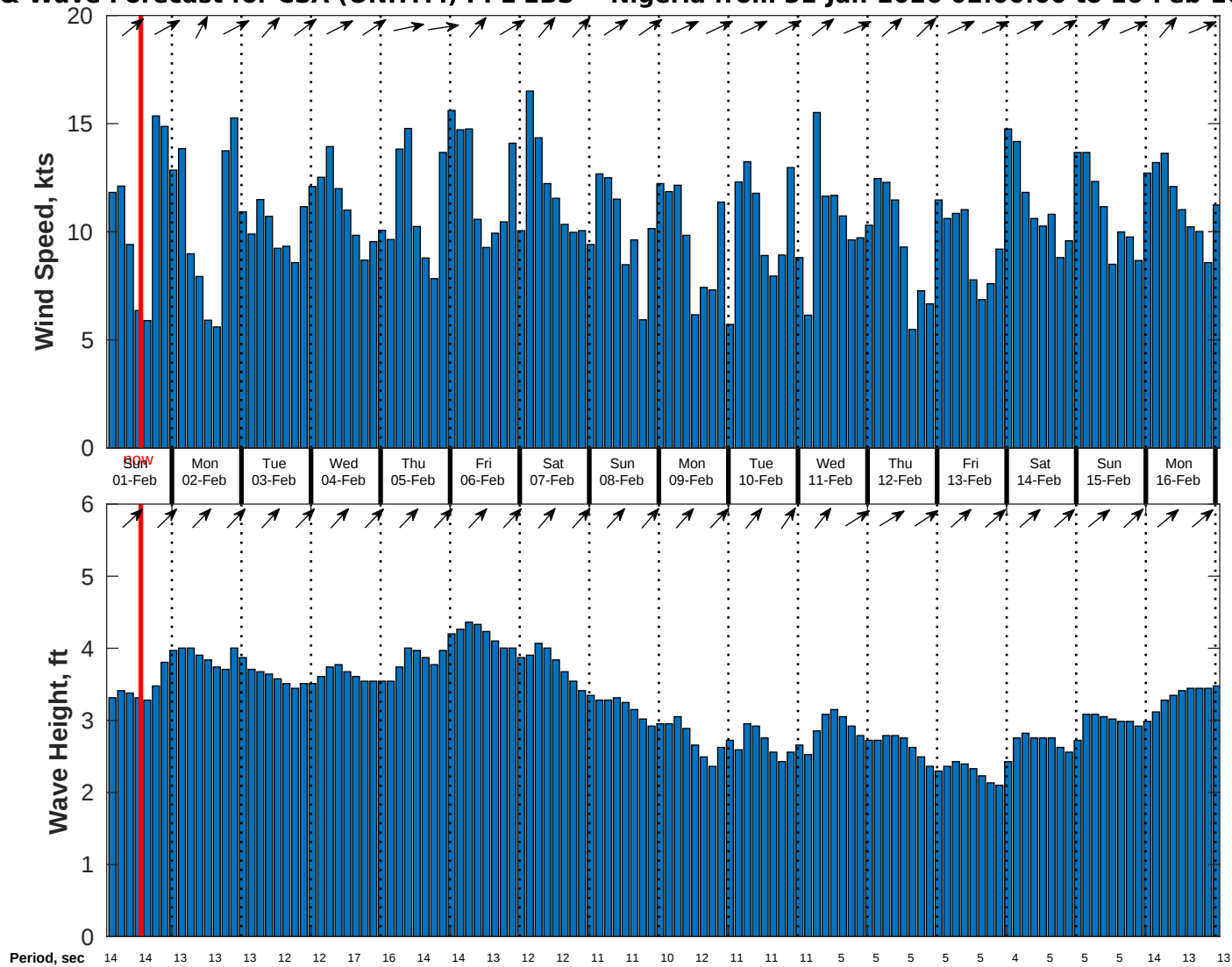
Wind & Wave Forecast for CSA (ONHYM) PPL EBS - Nigeria from 31-Jan-2026 02:00:00 to 16-Feb-2026 02:00:00
