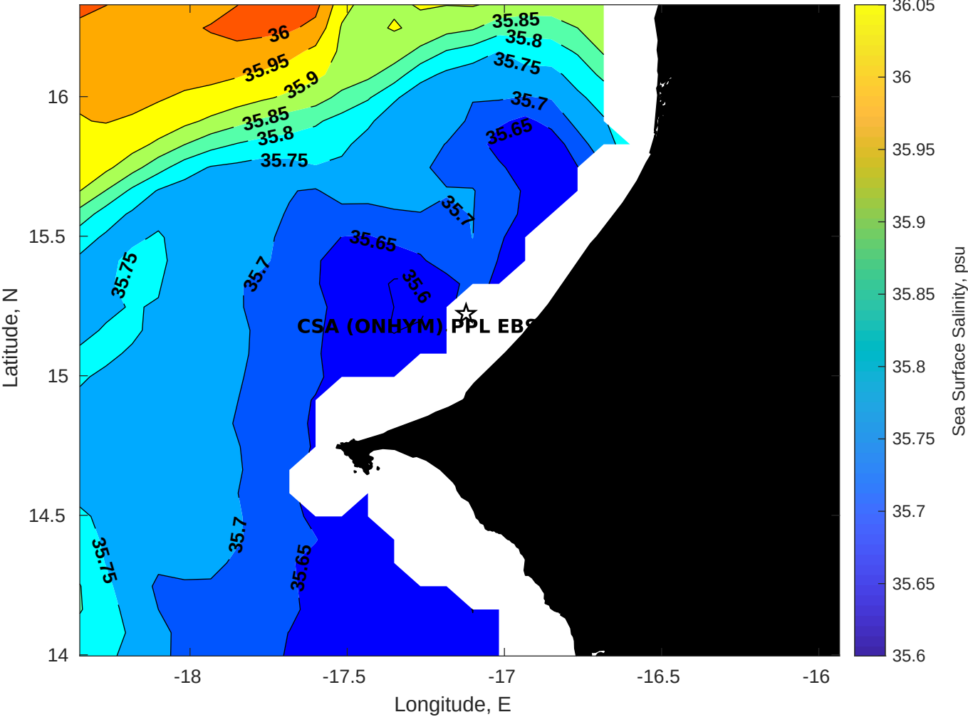
Surface Salinity for CSA (ONHYM) PPL EBS - Senegal at 30-Jan-2026 00:00:00
