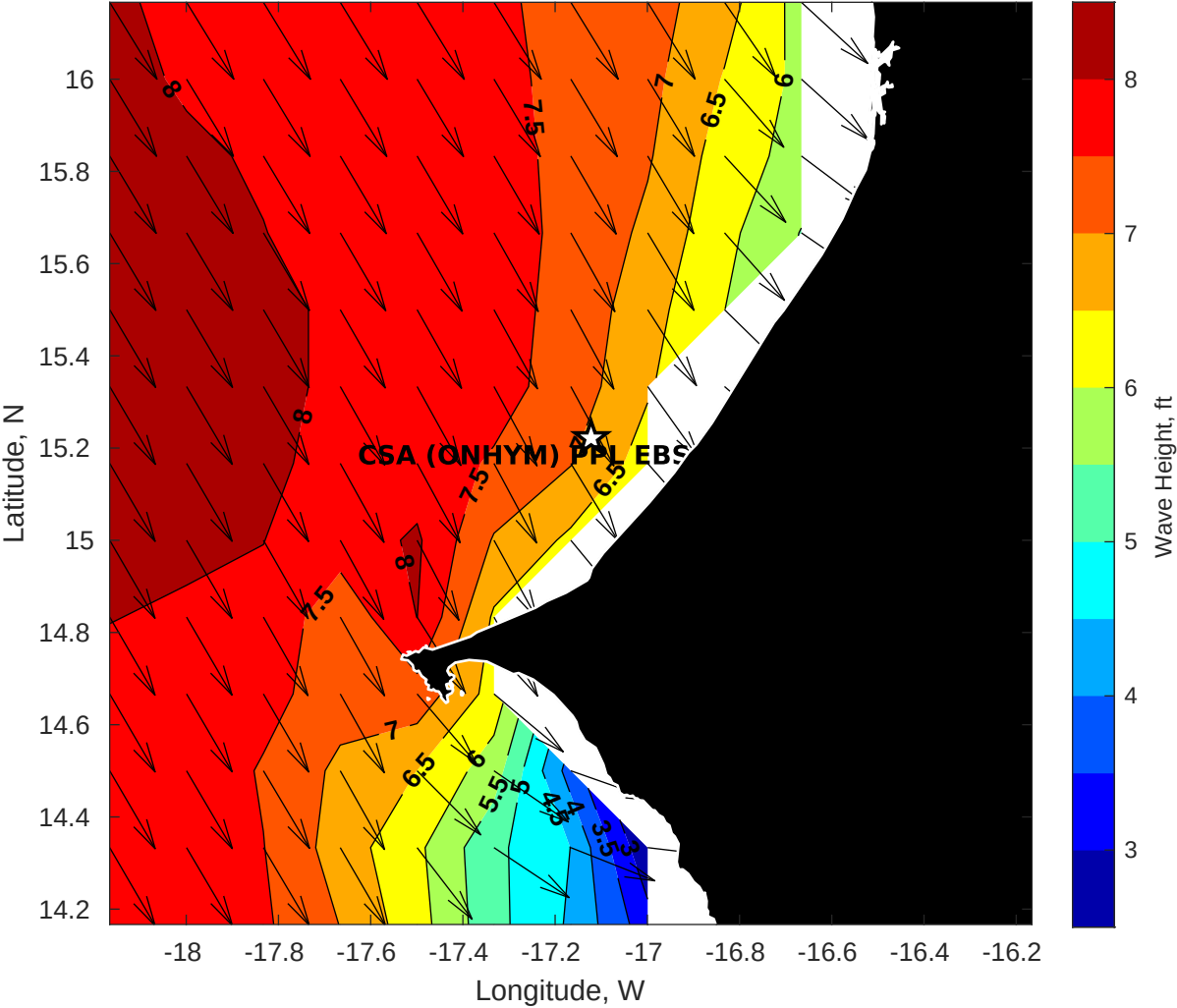
GFS Wave Height (ft) for CSA (ONHYM) PPL EBS - Senegal at 31-Jan-2026 09:00:00
