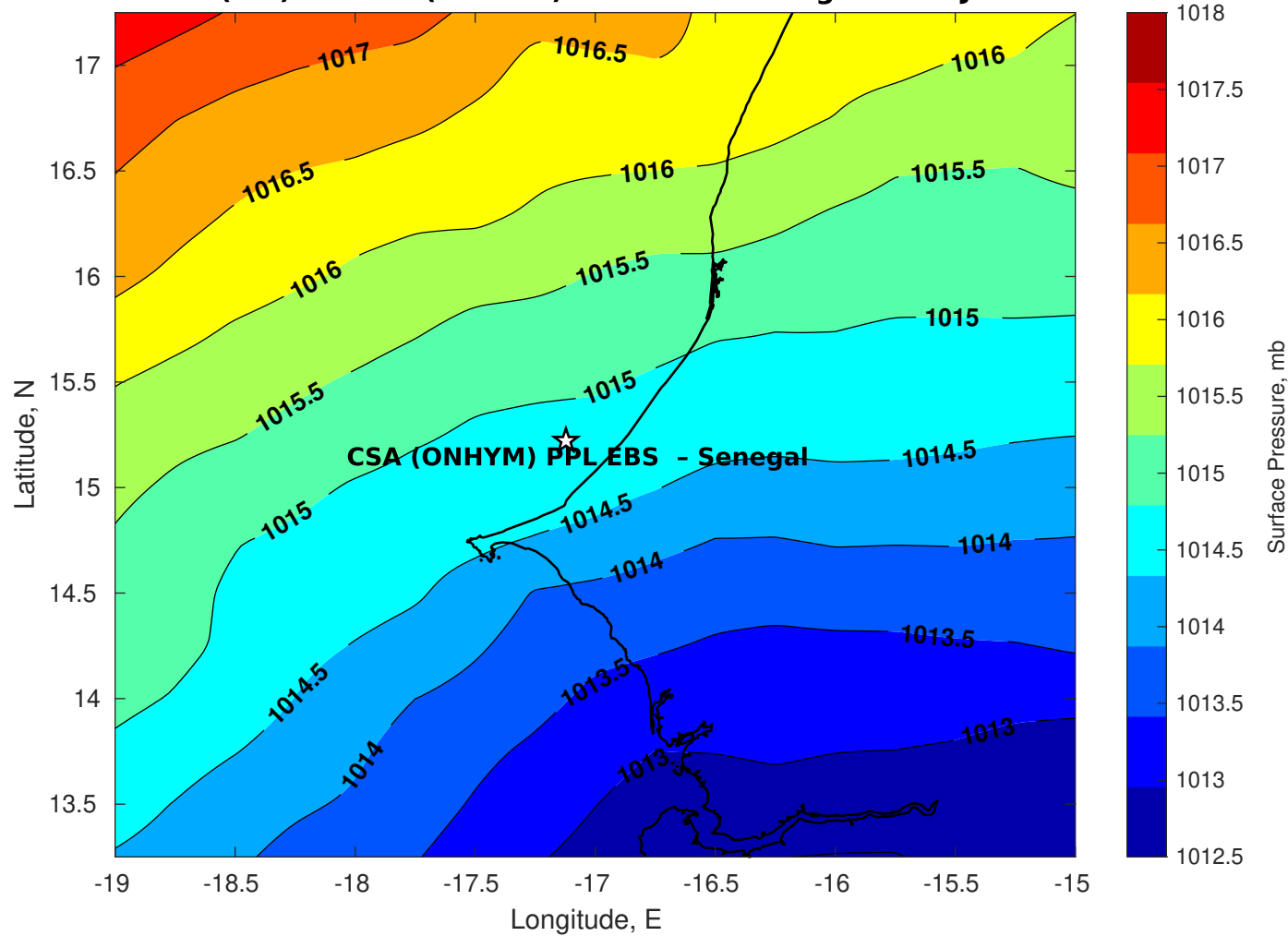
Surface Pressure (mb) for CSA (ONHYM) PPL EBS - Senegal at 31-Jan-2026 00:00:00
