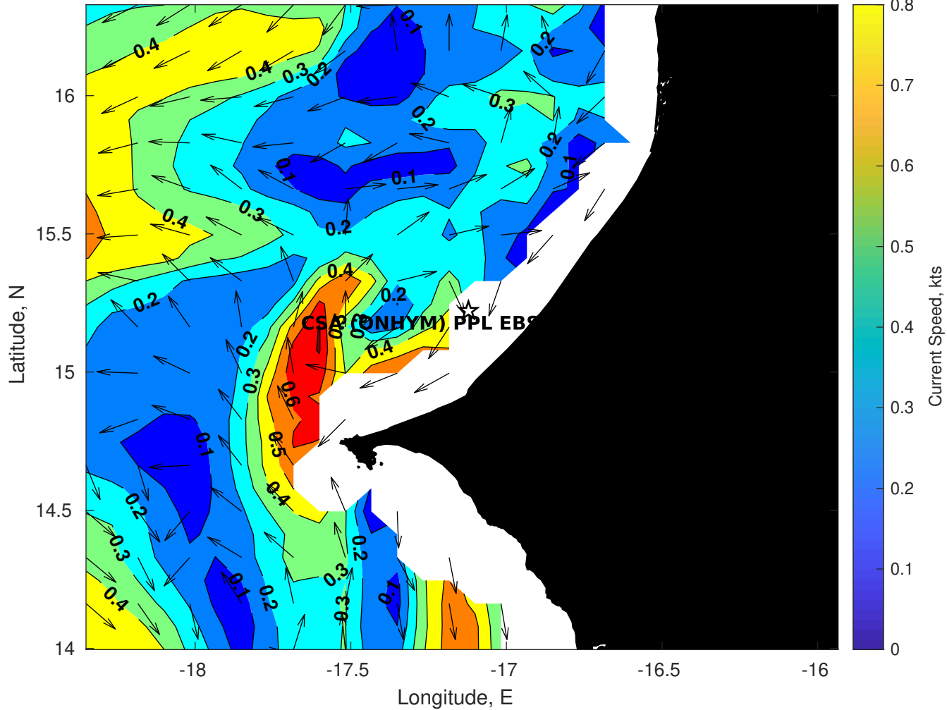
Surface Currents for CSA (ONHYM) PPL EBS - Senegal at 30-Jan-2026 00:00:00
