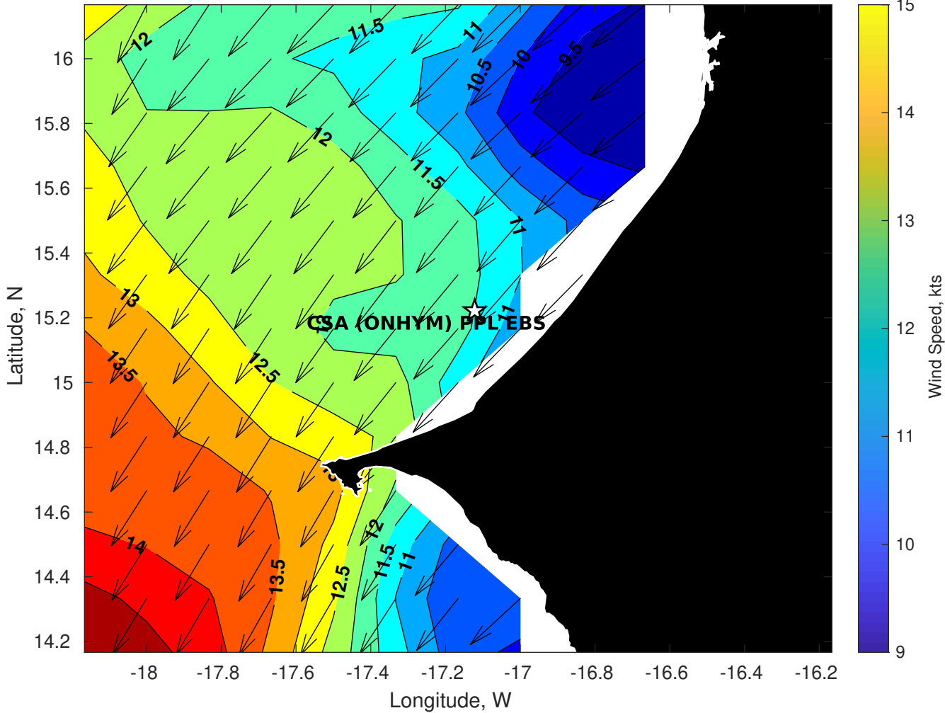
GFS Winds (kts) for CSA (ONHYM) PPL EBS - Senegal at 31-Jan-2026 09:00:00
