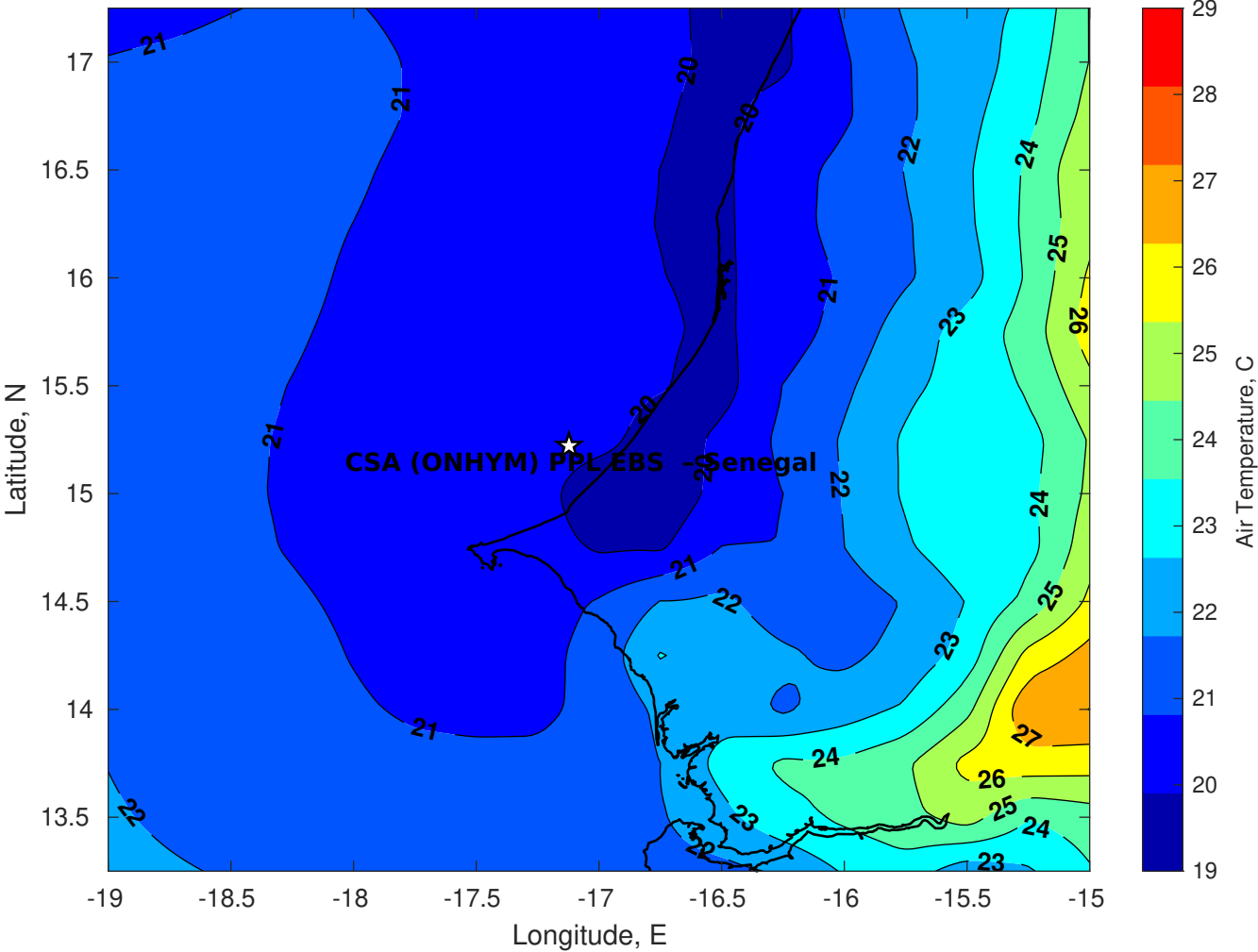
Air Temperature (C) for CSA (ONHYM) PPL EBS - Senegal at 31-Jan-2026
