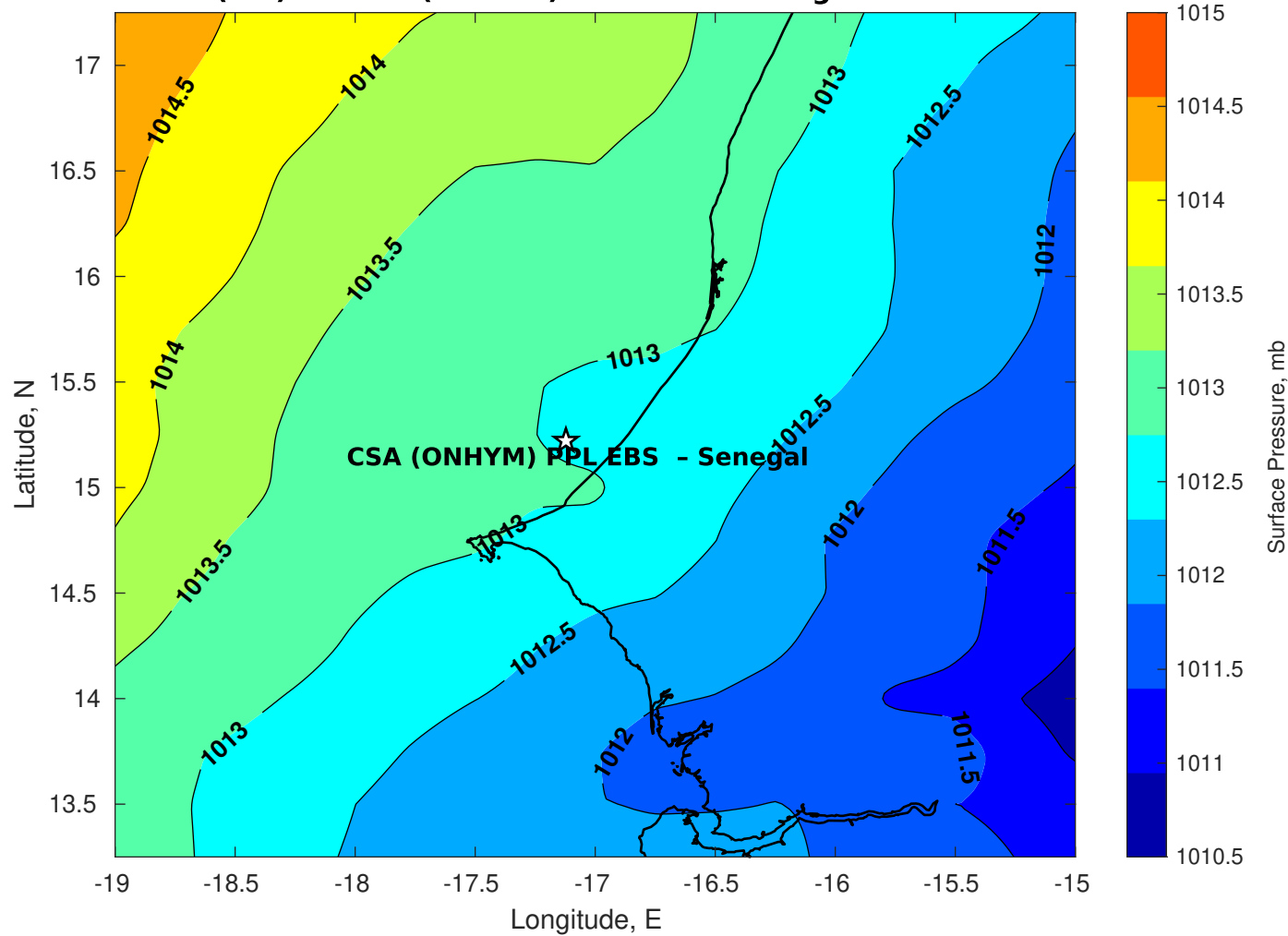
Surface Pressure (mb) for CSA (ONHYM) PPL EBS - Senegal at 02-Feb-2026 00:00:00
