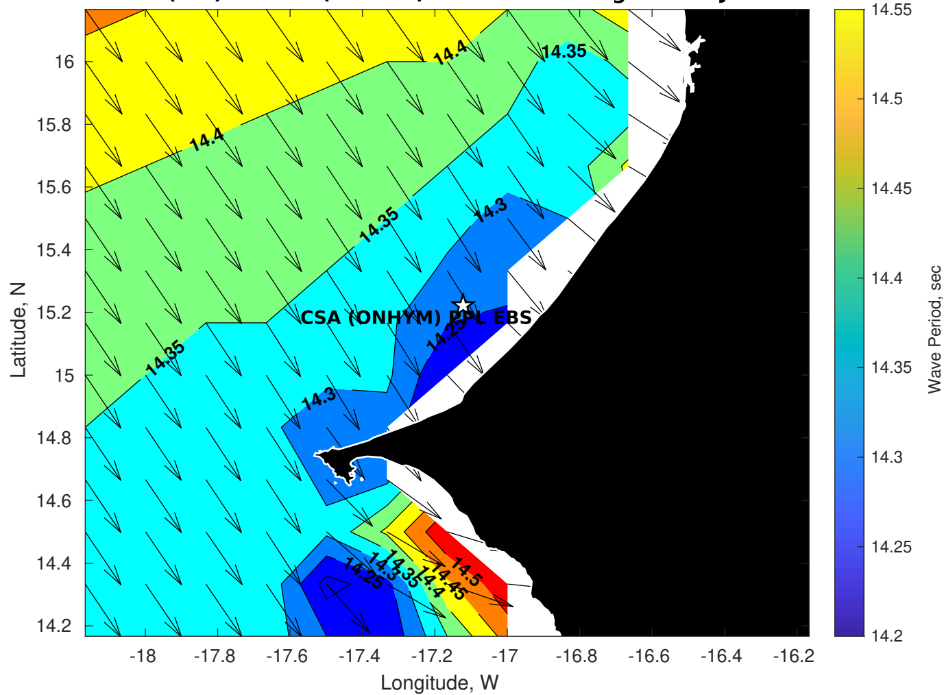
GFS Wave Period (sec) for CSA (ONHYM) PPL EBS - Senegal at 31-Jan-2026 09:00:00
