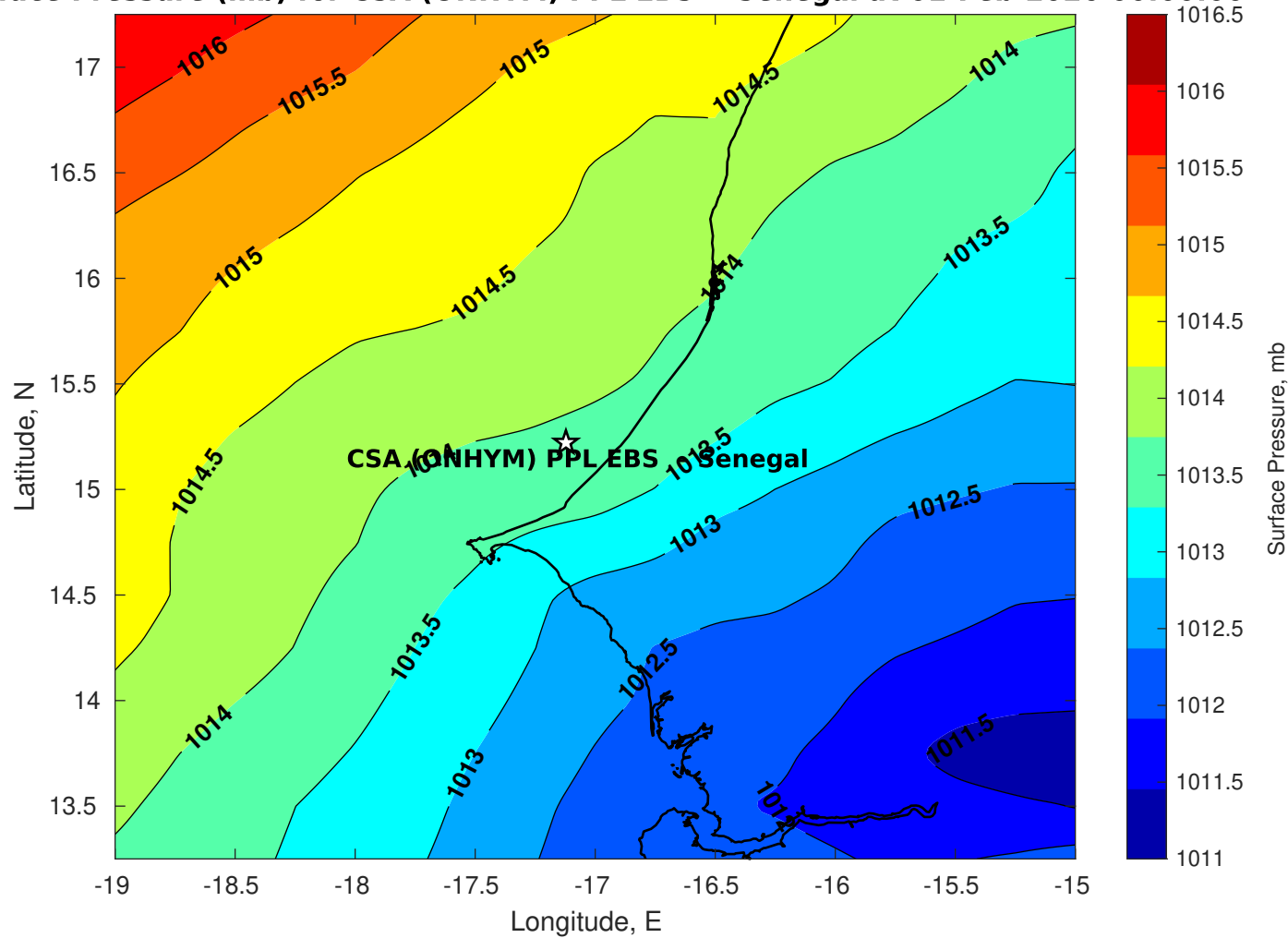
Surface Pressure (mb) for CSA (ONHYM) PPL EBS - Senegal at 01-Feb-2026 00:00:00
