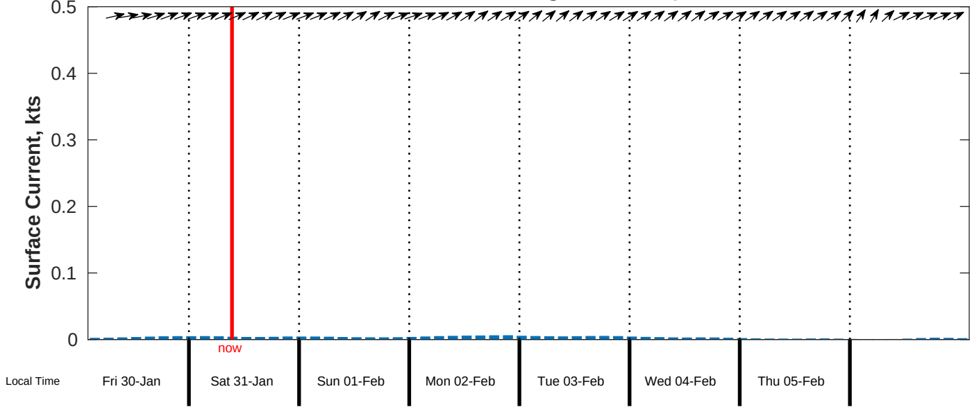
Surface Current Forecast for CSA (ONHYM) PPL EBS - Senegal from 30-Jan-2026 00:00:00 to 07-Feb-2026 00:00:00
