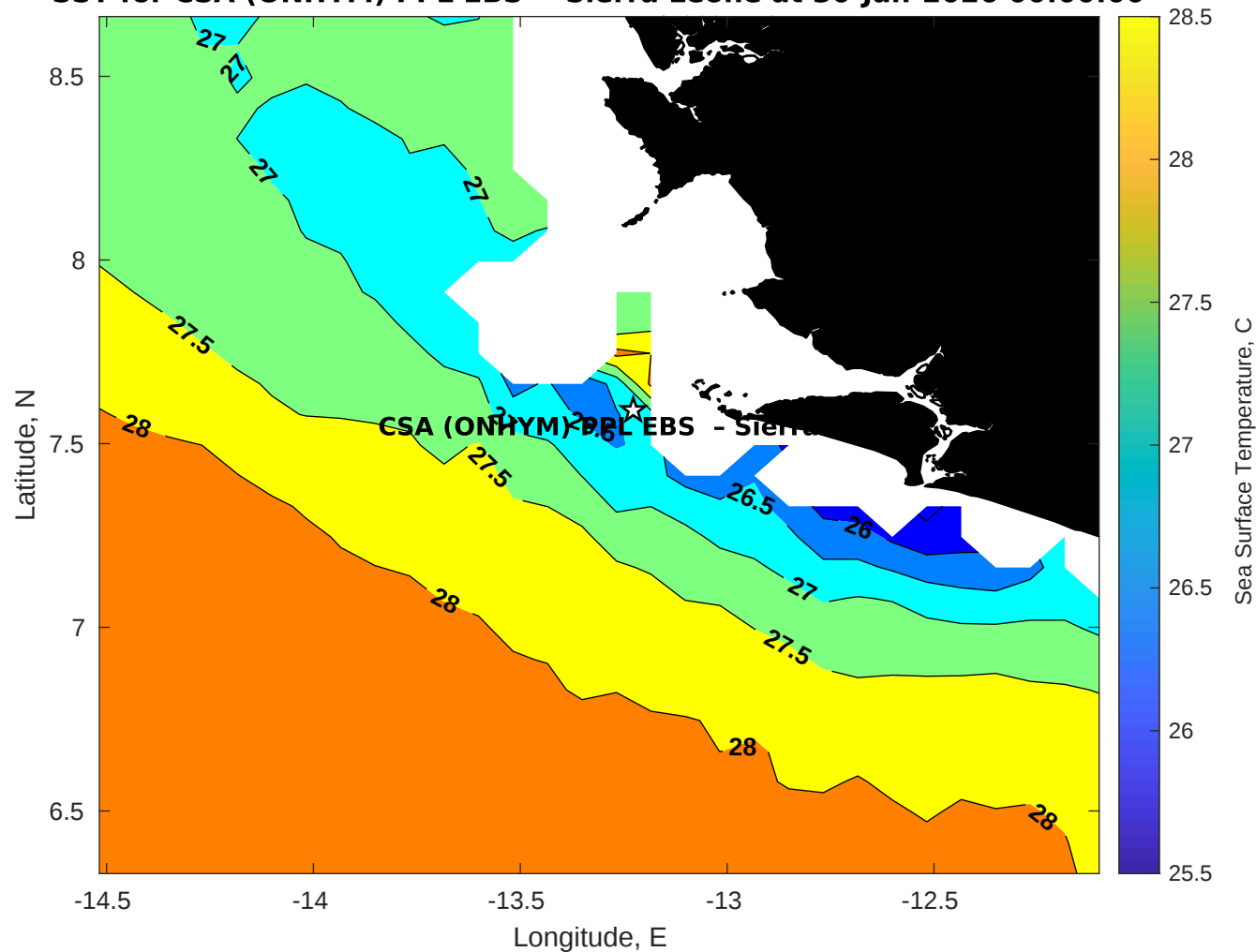
SST for CSA (ONHYM) PPL EBS - Sierra Leone at 30-Jan-2026 00:00:00
