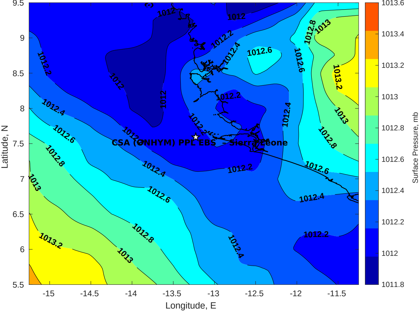
Surface Pressure (mb) for CSA (ONHYM) PPL EBS - Sierra Leone at 31-Jan-2026 00:00:00
