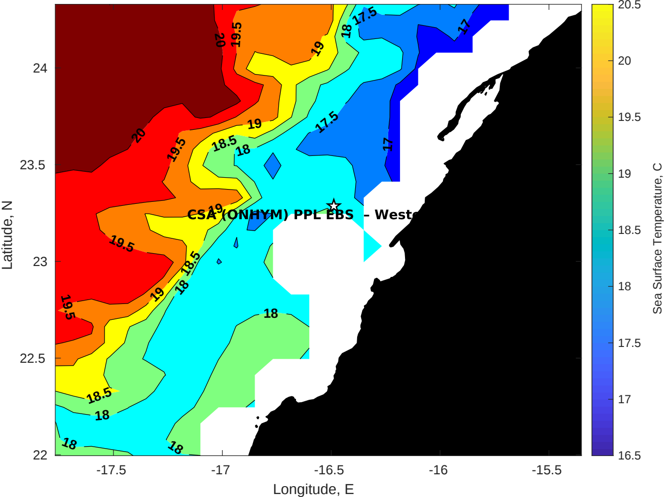
SST for CSA (ONHYM) PPL EBS - Western Sahara at 30-Jan-2026 00:00:00
