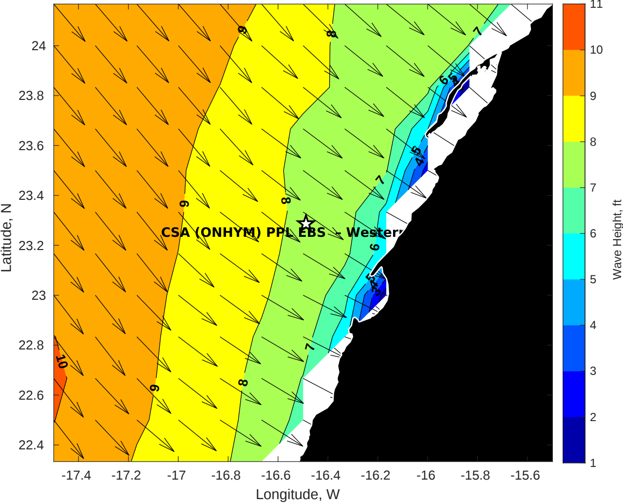
GFS Wave Height (ft) for CSA (ONHYM) PPL EBS - Western Sahara at 31-Jan-2026 09:00:00
