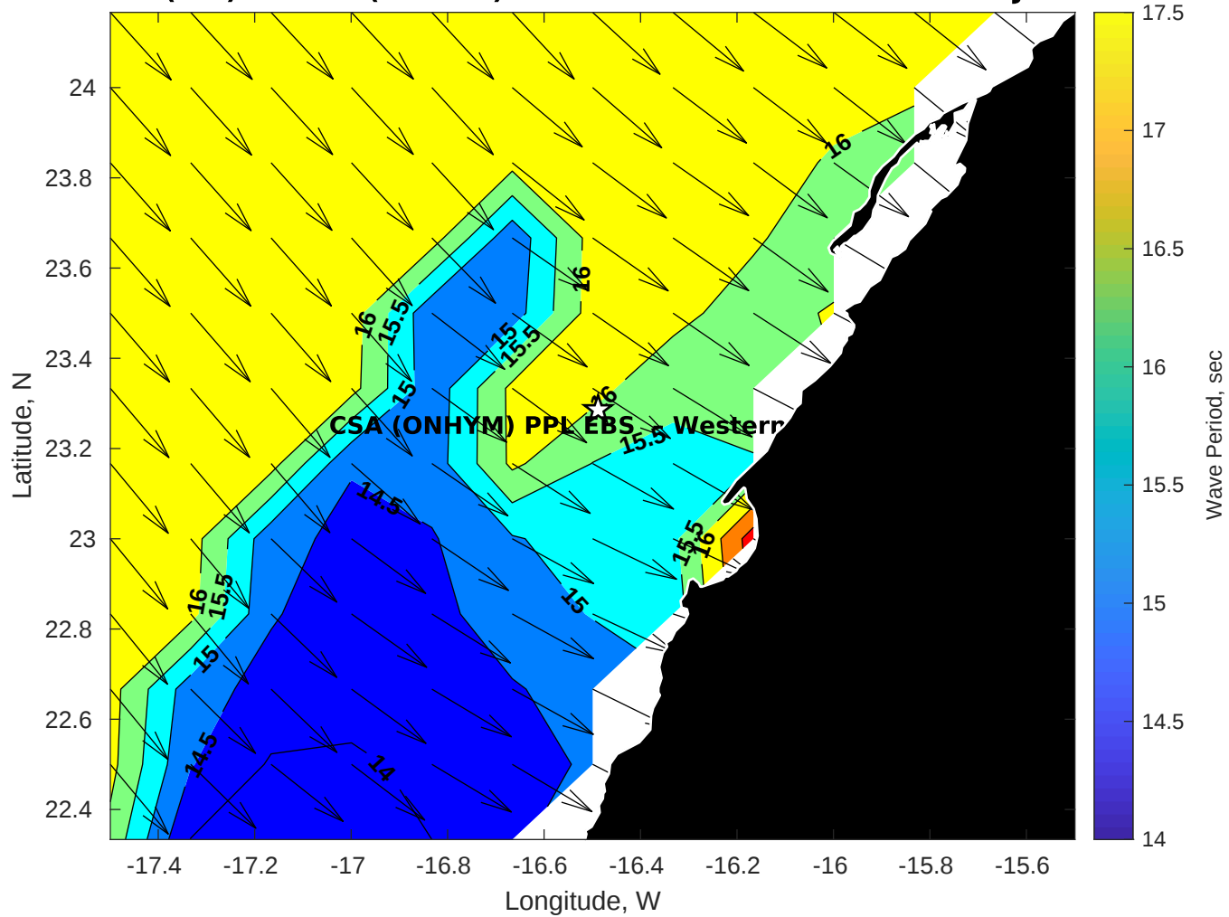
GFS Wave Period (sec) for CSA (ONHYM) PPL EBS - Western Sahara at 31-Jan-2026 09:00:00
