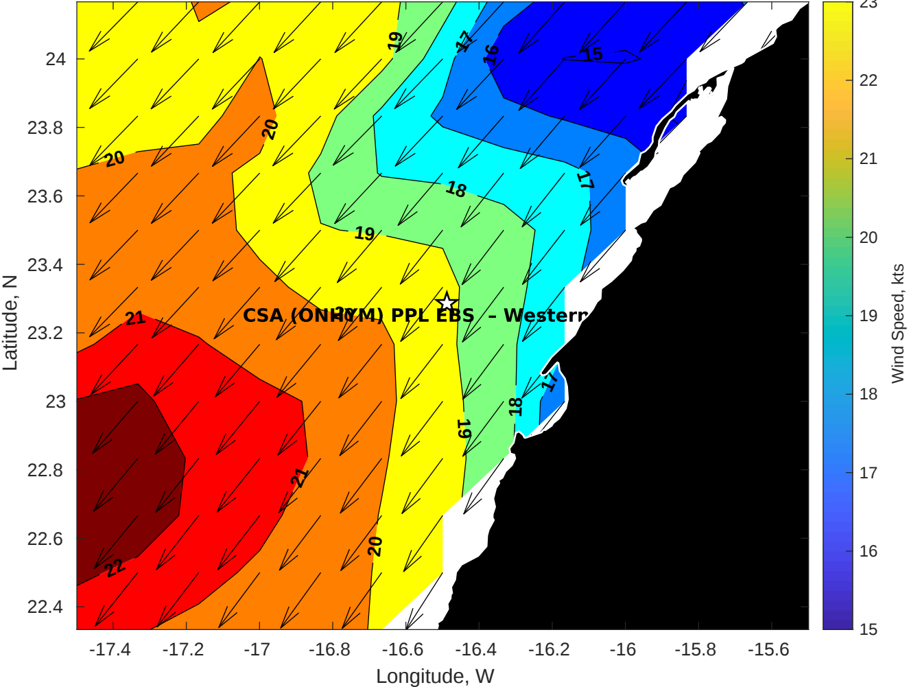
GFS Winds (kts) for CSA (ONHYM) PPL EBS - Western Sahara at 31-Jan-2026 09:00:00
