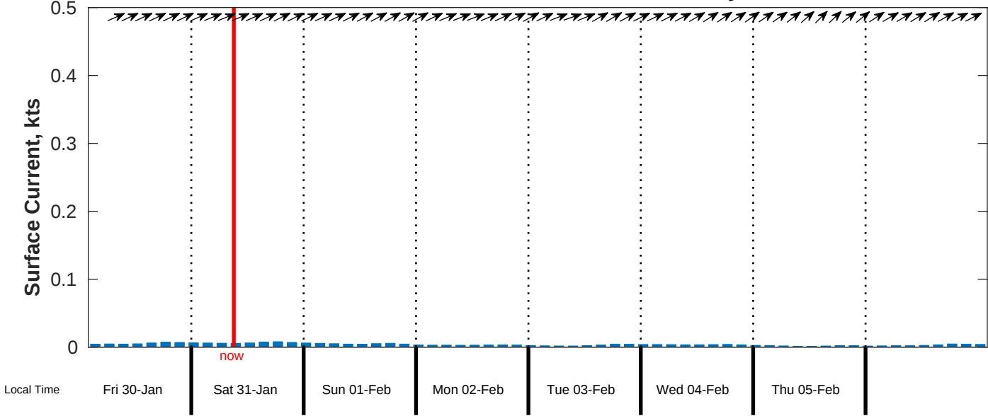
Surface Current Forecast for CSA (ONHYM) PPL EBS - Western Sahara from 30-Jan-2026 00:00:00 to 07-Feb-2026 00:00:00
