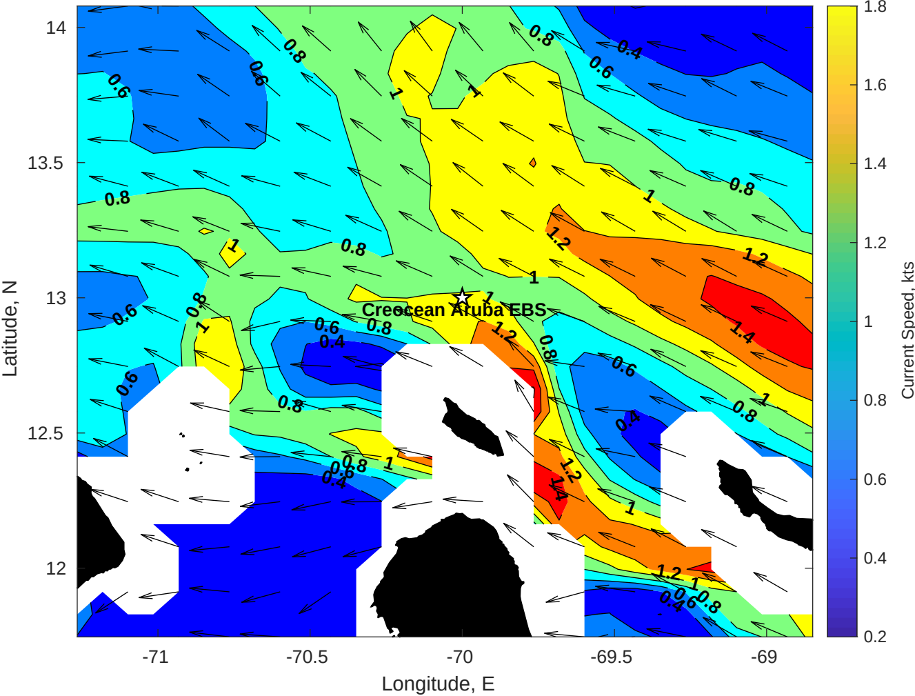
Surface Currents for Creoecean Aruba EBS at 30-Jan-2026 00:00:00
