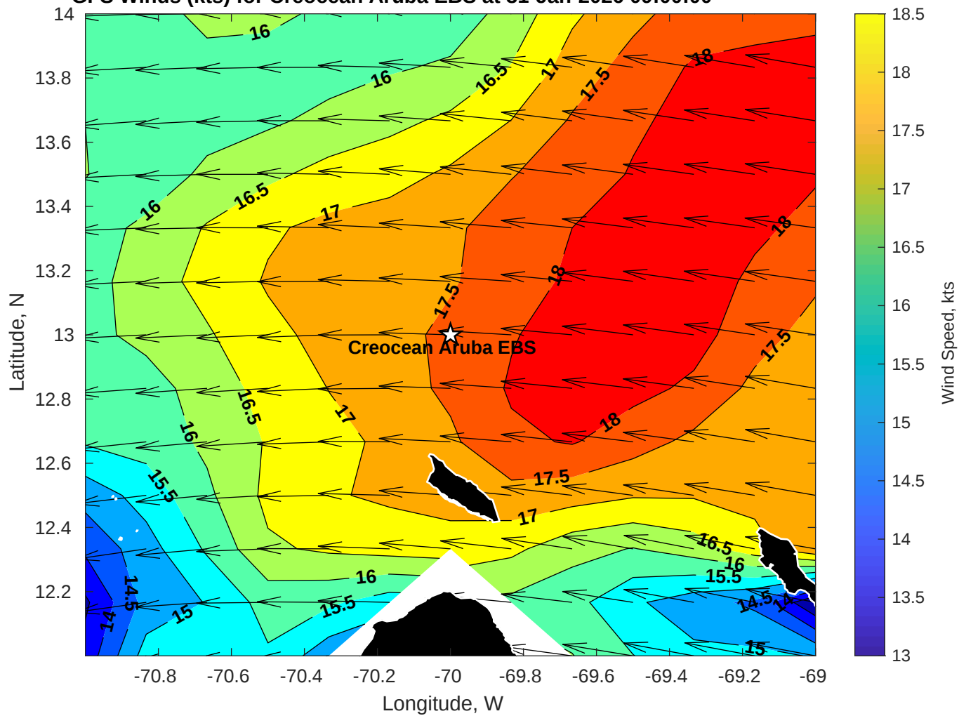
GFS Winds (kts) for Creoccean Aruba EBS at 31-Jan-2026 09:00:00
