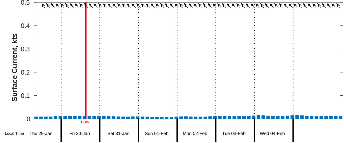
Surface Current Forecast for Creocean Aruba EBS from 30-Jan-2026 00:00:00 to 07-Feb-2026 00:00:00
