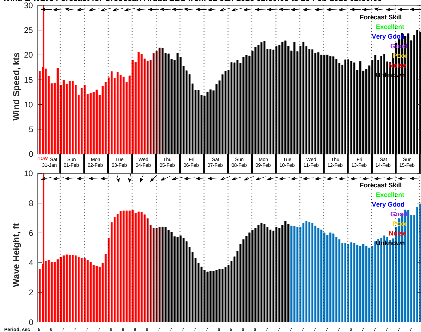
Wind & Wave Forecast for Creocan Aruba EBS from 31-Jan-2026 02:00:00 to 16-Feb-2026 02:00:00
