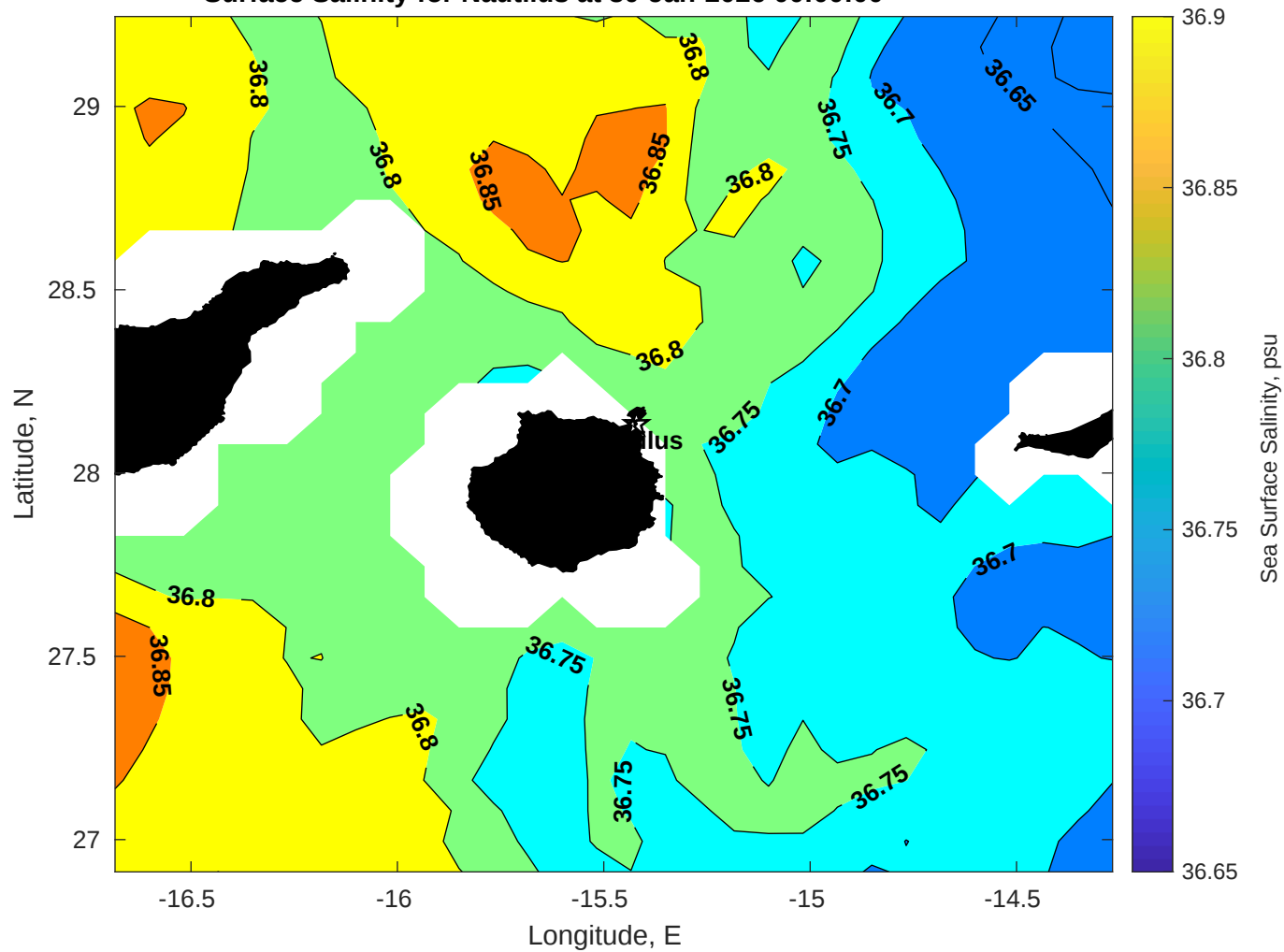
Surface Salinity for Nautilus at 30-Jan-2026 00:00:00
