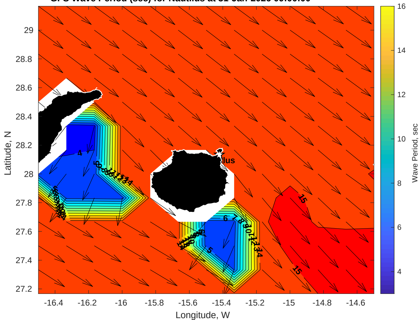
GFS Wave Period (sec) for Nautilus at 31-Jan-2026 09:00:00
