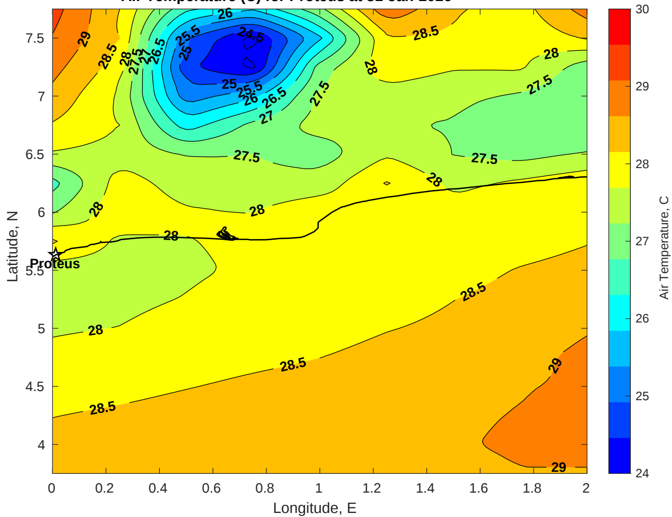
Air Temperature (C) for Proteus at 31-Jan-2026
