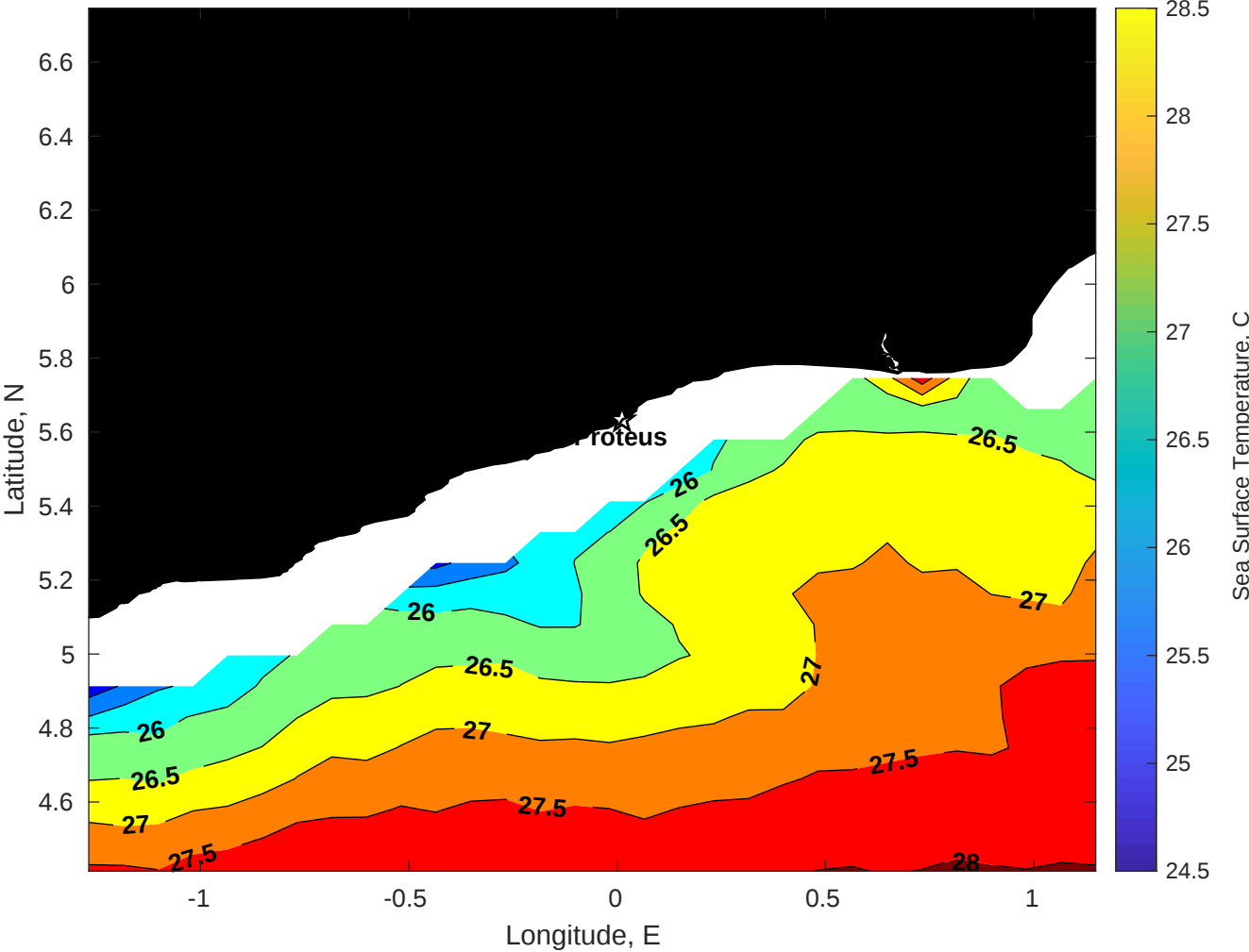
SST for Proteus at 30-Jan-2026 00:00:00
