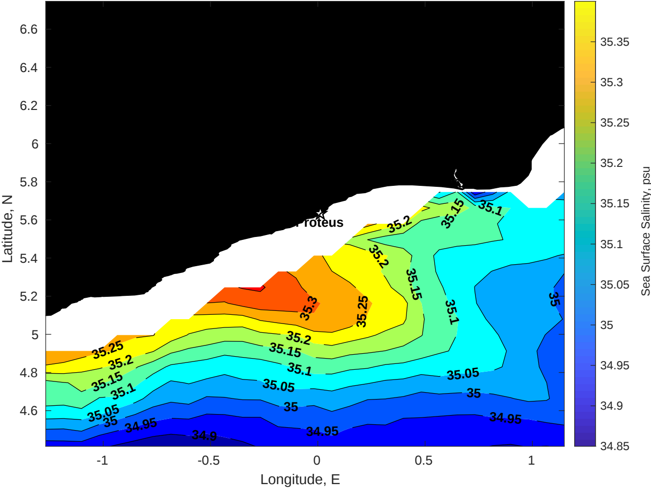
Surface Salinity for Proteus at 30-Jan-2026 00:00:00
