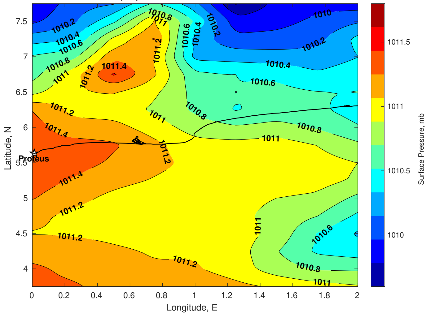
Surface Pressure (mb) for Proteus at 02-Feb-2026 00:00:00
