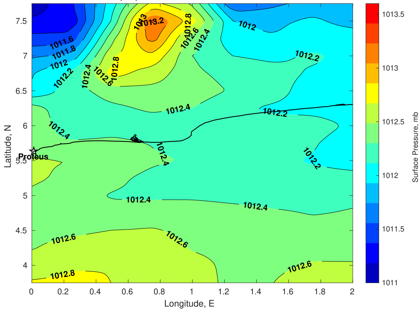
Surface Pressure (mb) for Proteus at 31-Jan-2026 00:00:00
