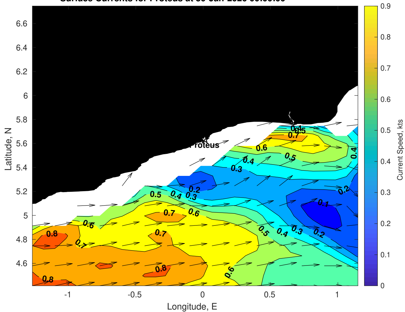
Surface Currents for Proteus at 30-Jan-2026 00:00:00
