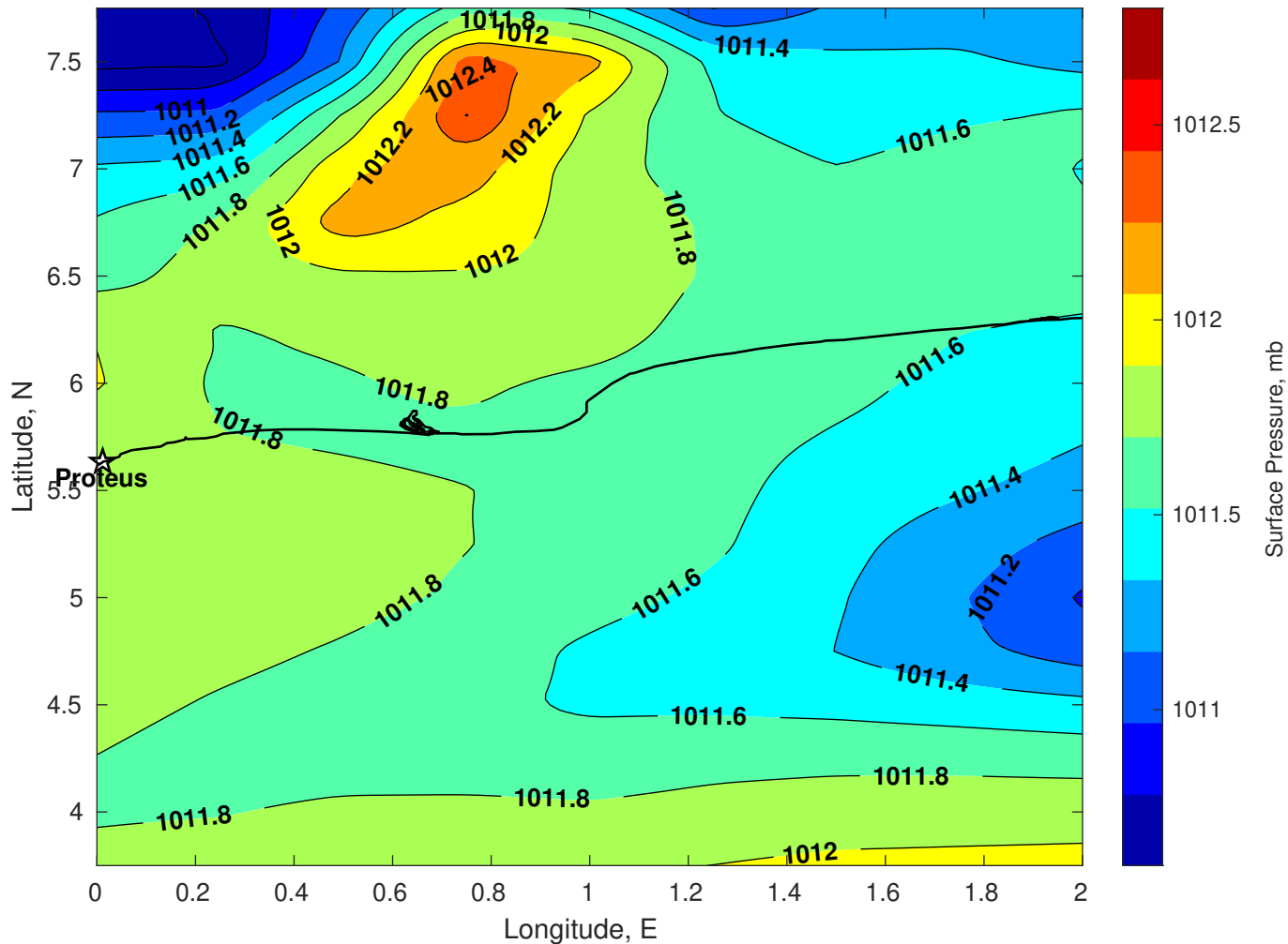
Surface Pressure (mb) for Proteus at 01-Feb-2026 00:00:00
