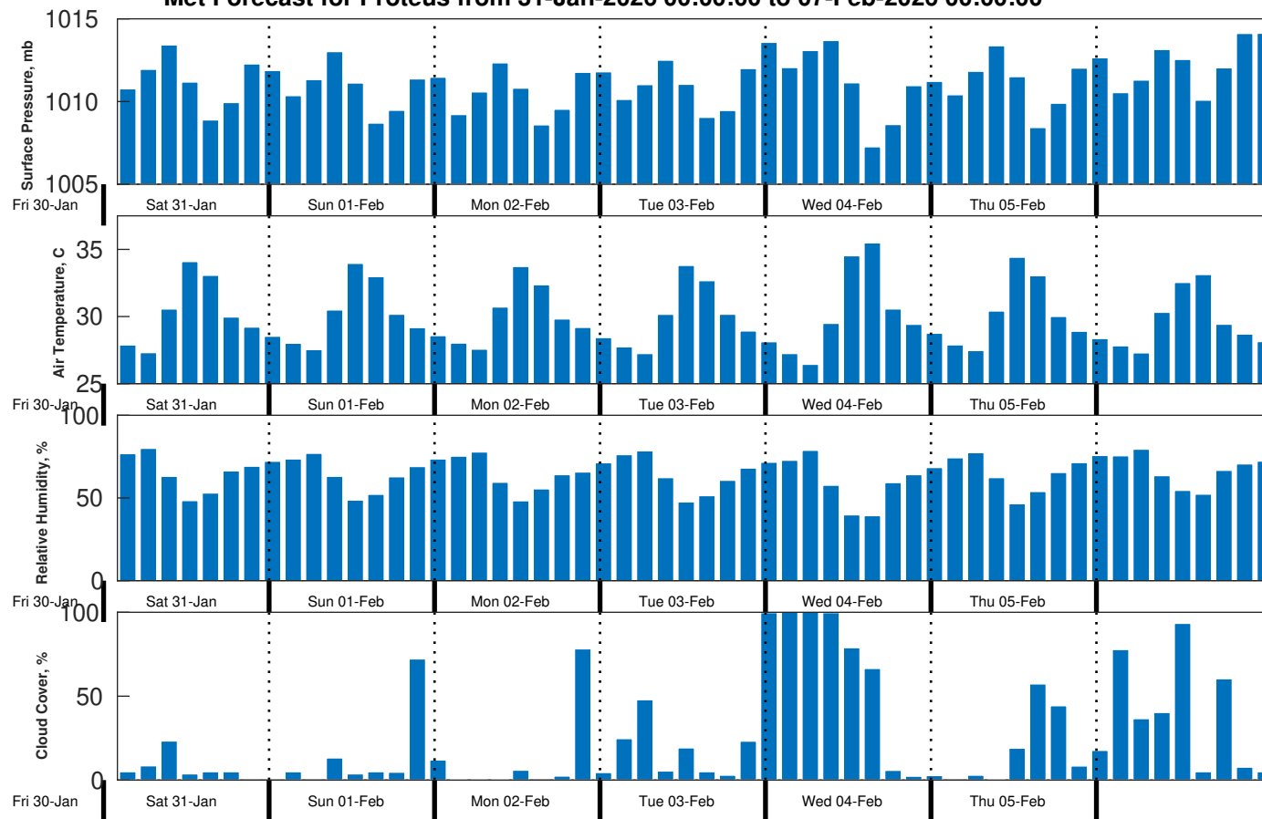
Met Forecast for Proteus from 31-Jan-2026 00:00:00 to 07-Feb-2026 00:00:00
